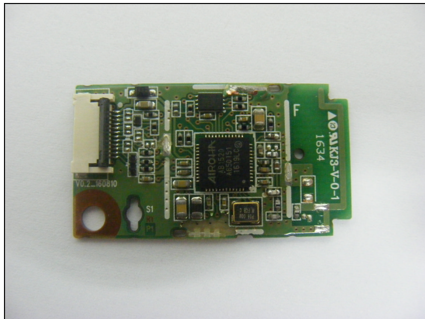
Top view of main board (Shielding can off)
