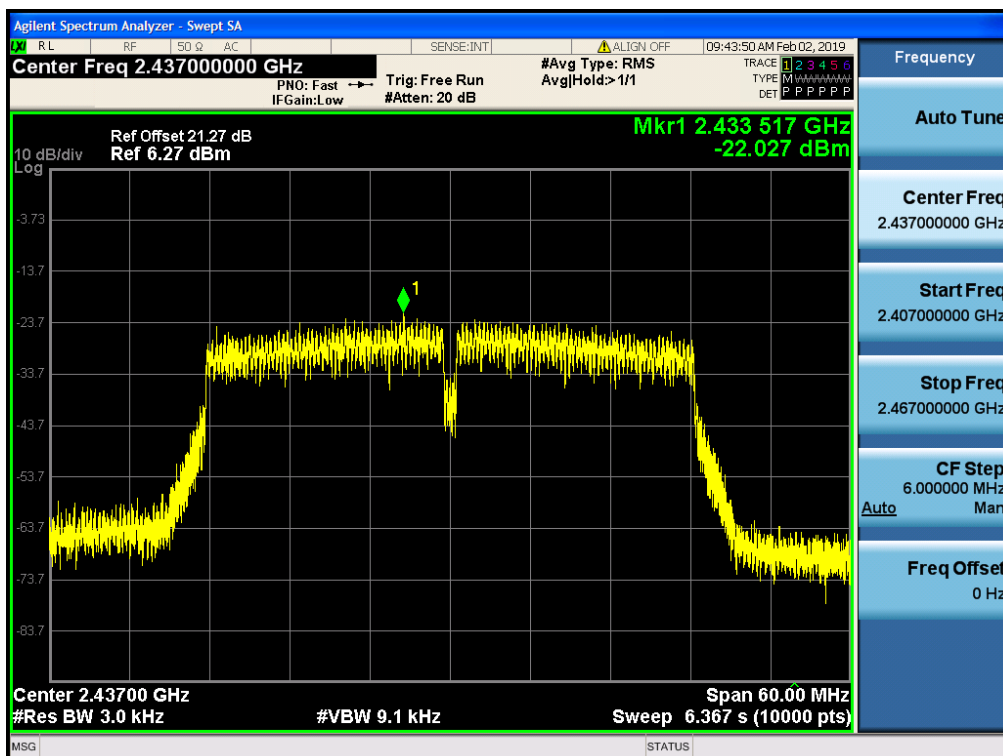
Power Spectral Density (802.11n_HT40 -CH 6)
