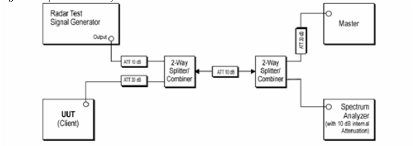
Figure 1. Setup for Client with injection at the Master
