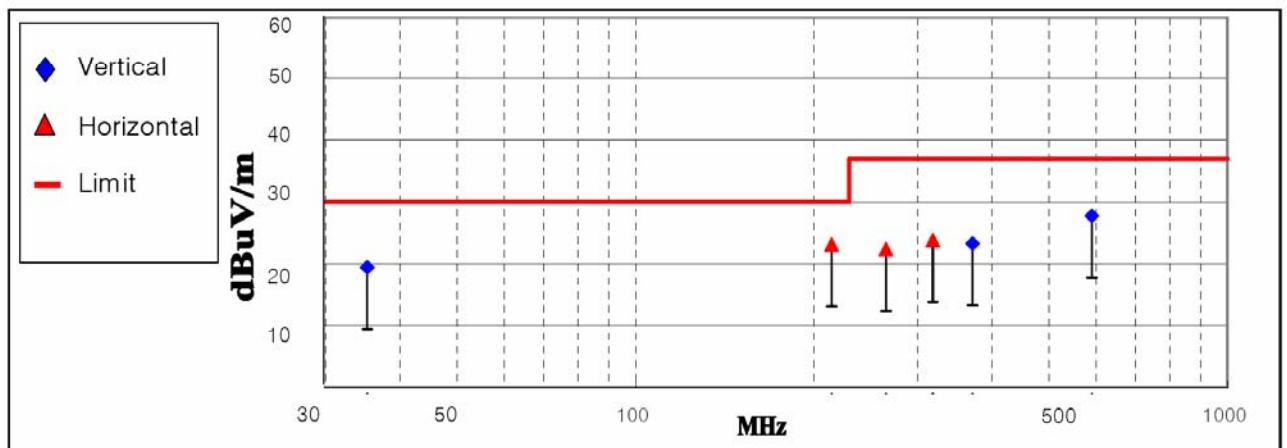
< Fig 4. Radiated emission result >
