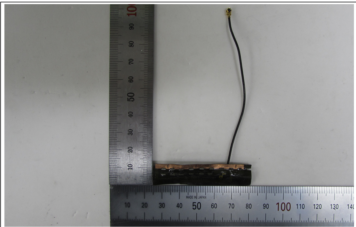
<Main Antenna>
