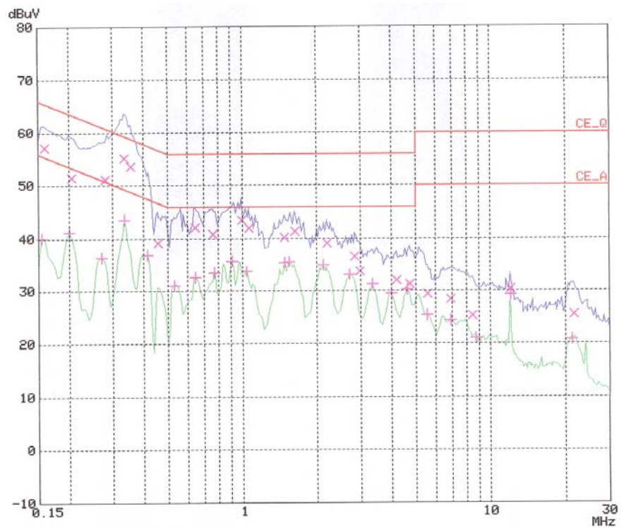
< Neutral line >
