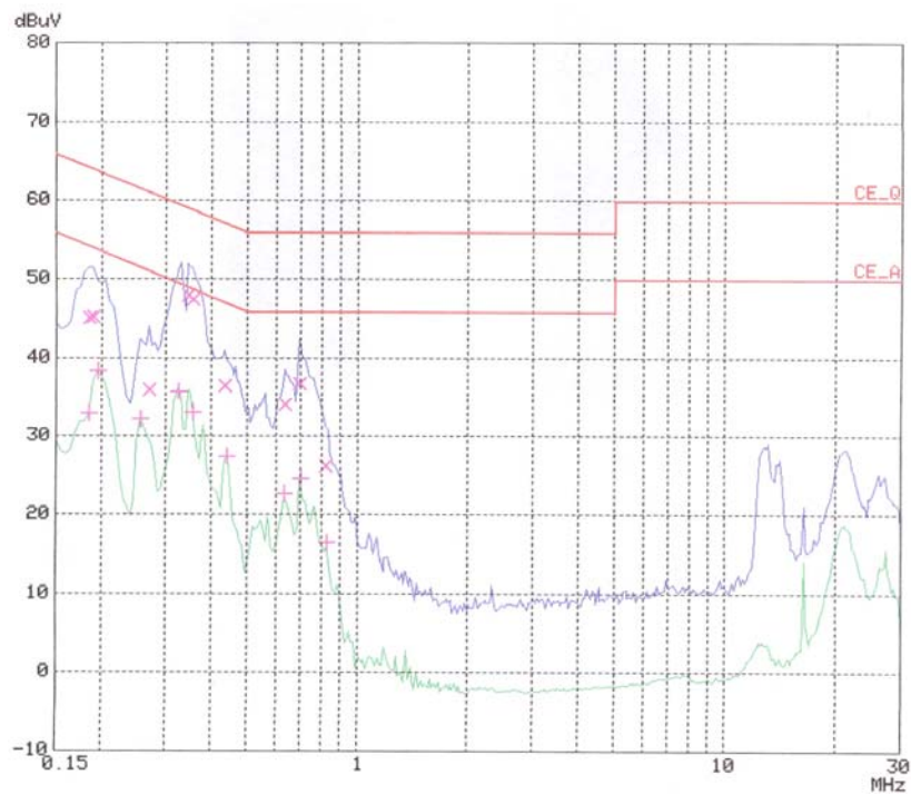
< Hot line >
