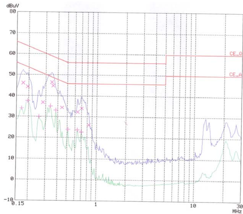
< Neutral line >
