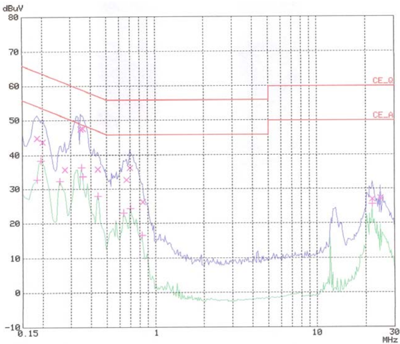
< Hot line >
