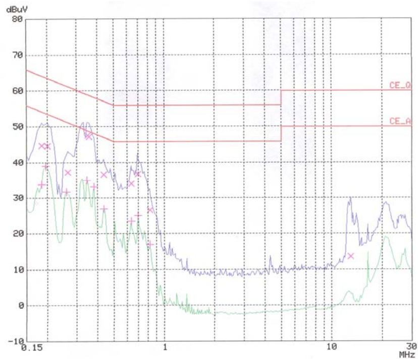
< Neutral line >
