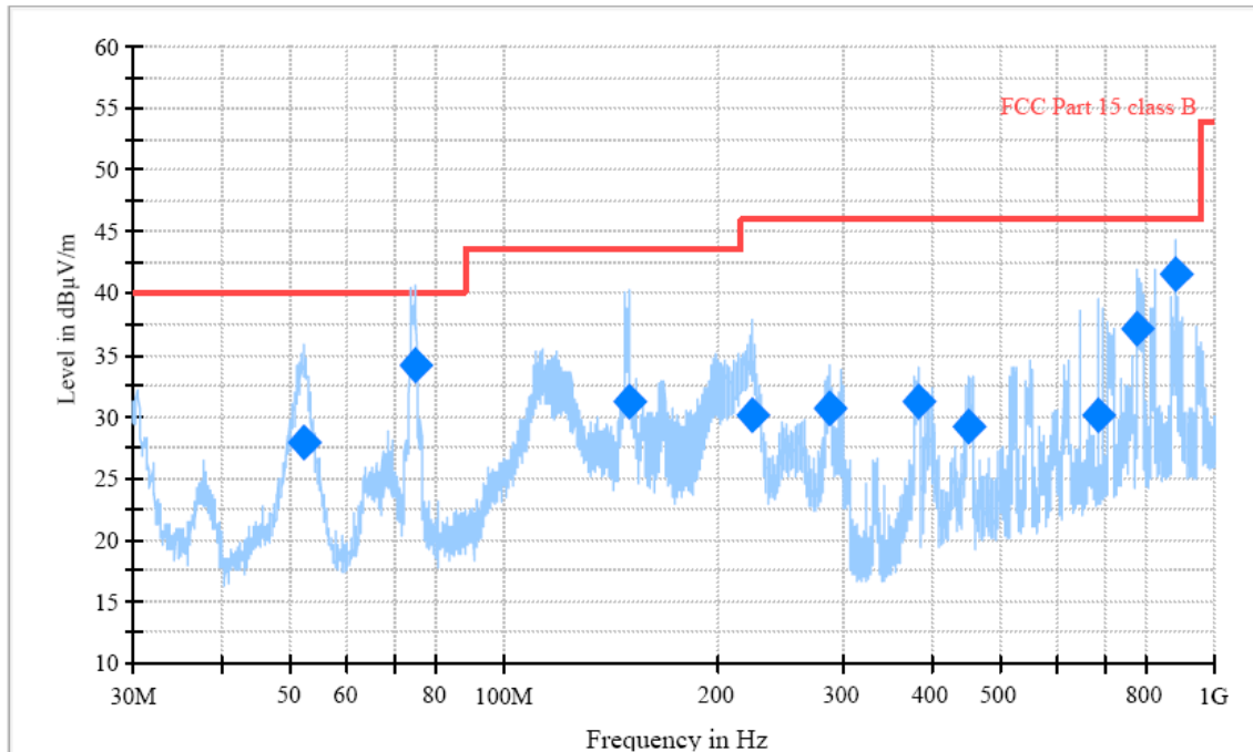
ESIB_Direct_Electric Field Strength
