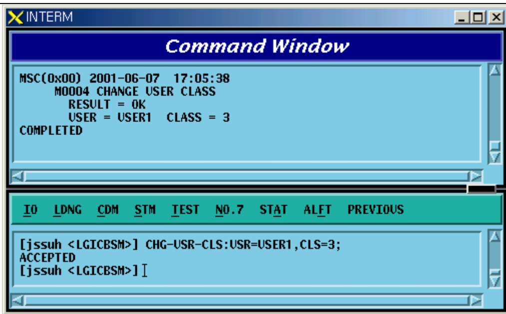
Fig. 4.1-8 User Class Change
