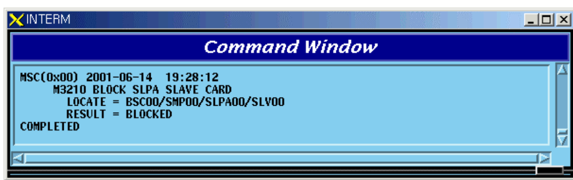
Fig. 4.4-24 Result of SLPA BLOCK Command
