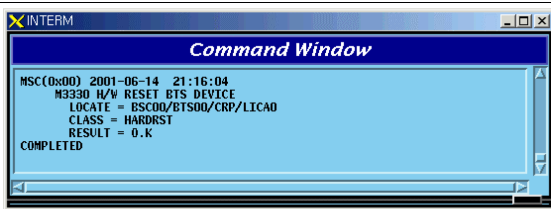
Fig. 4.4-38 Result of H/W RESET BTS Device Command
