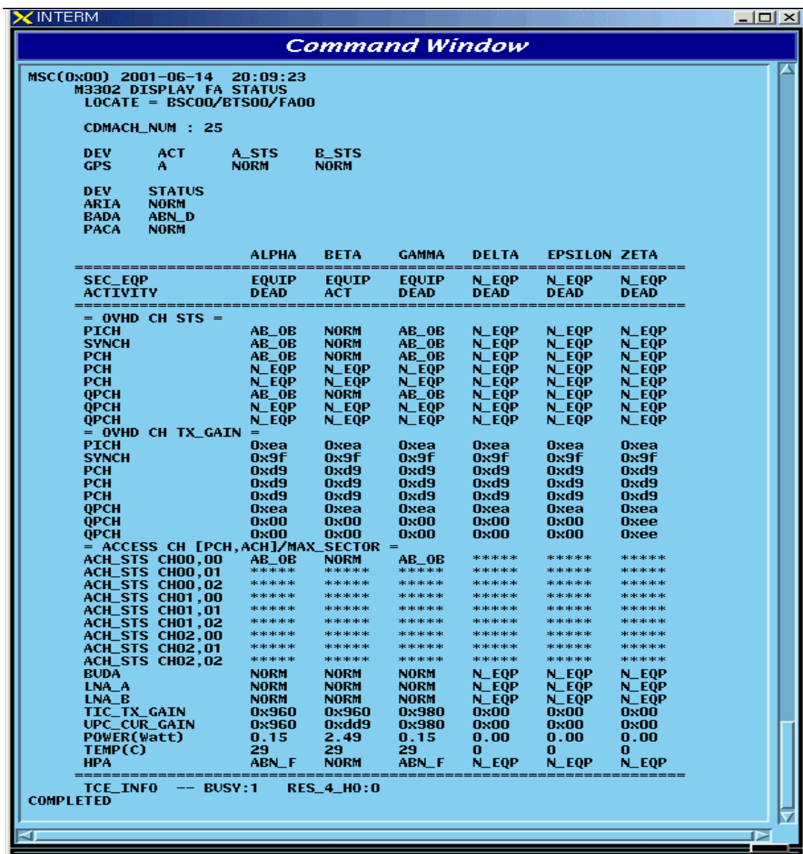
Fig. 4.4-33 Result of FA Status Display Command
