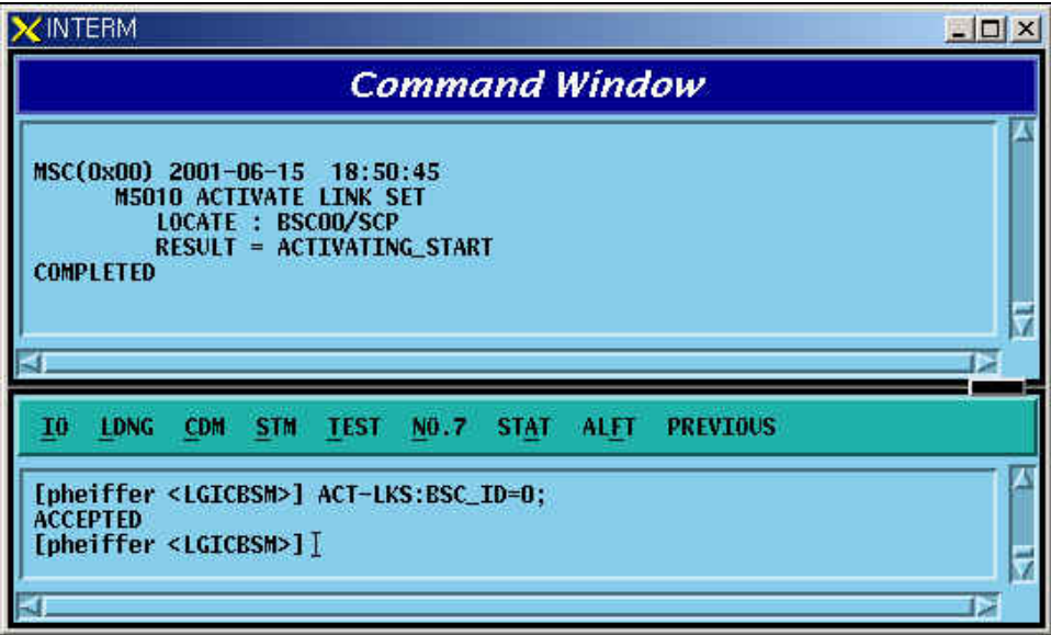
Fig. 4.6-4 Activation of Signaling Link Set
