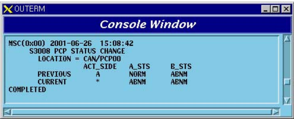
Fig. 5.2-3 PCP Processor Status Change Report
