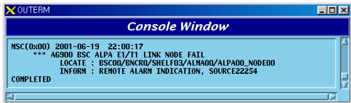
Fig. 5.1-140 ASLB ALPA Link Fail((RAI)
