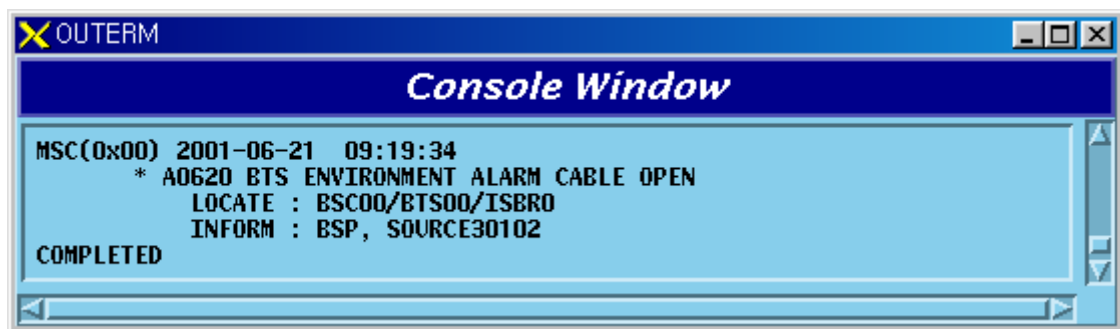
Fig. 5.1-241 Outdoor BTS ENV Rectifier Unit Alarm Cable Open
