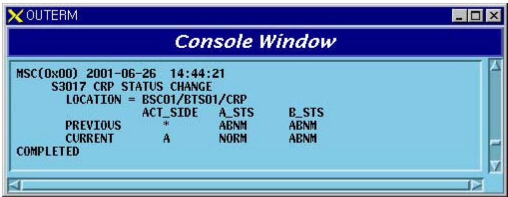
Fig. 5.2-12 CRP Processor Status Change Report
