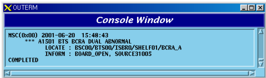
Fig. 5.1-183 BANB BCRA Dual Board Open Fail
