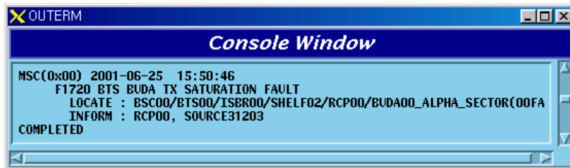
Fig. 5.1-360 BUDA Tx Saturation Fault
