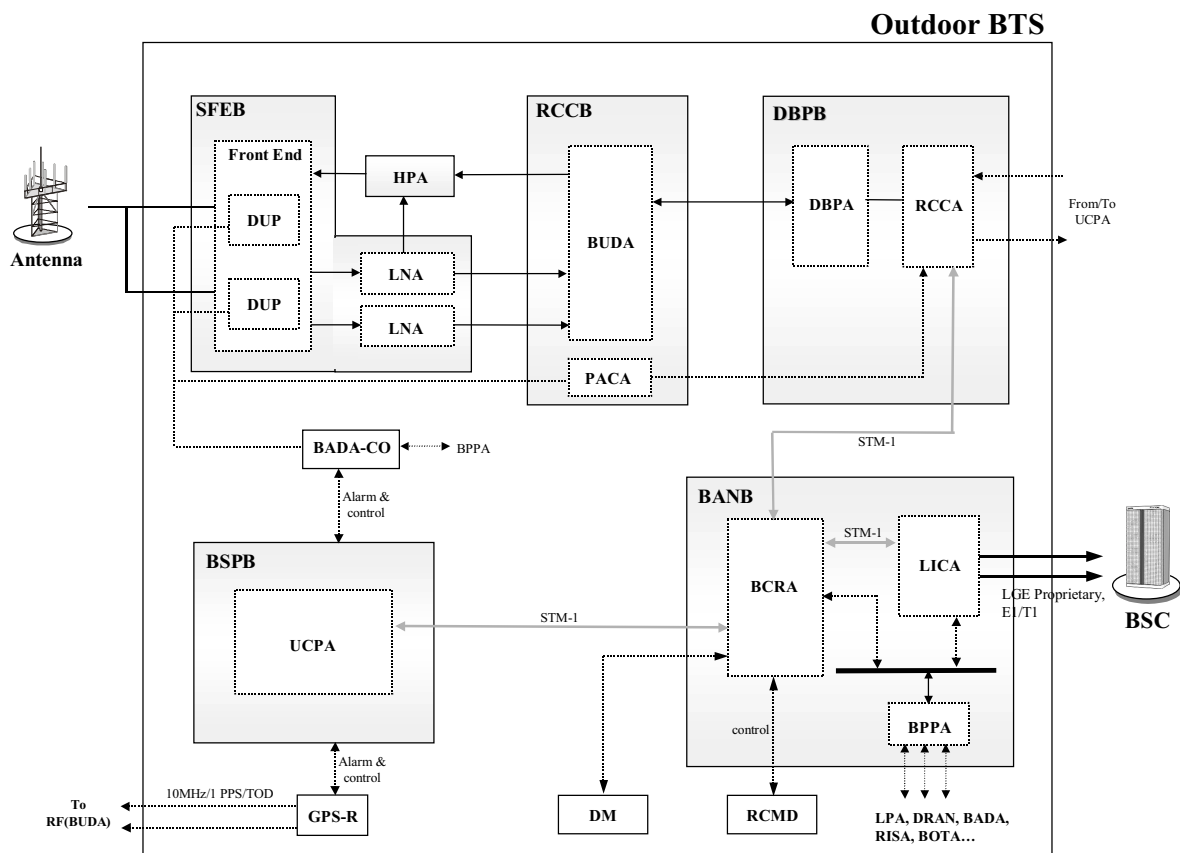
Figure 2-1 Outdoor BTS H/W configuration
