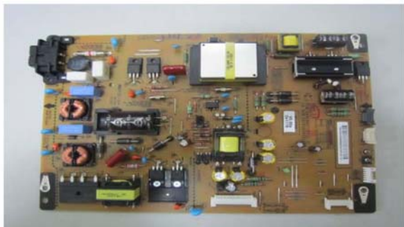
POWER BOARD FRONT(before)
