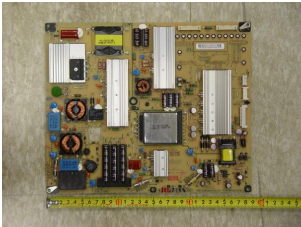
Original (LG Electronics Inc. / LGP4247-11SLPB)
