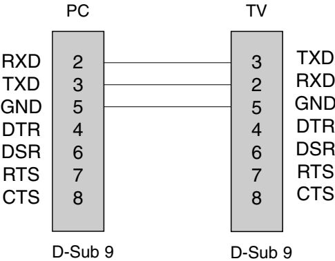
3-Wire Configurations (Not standard)
