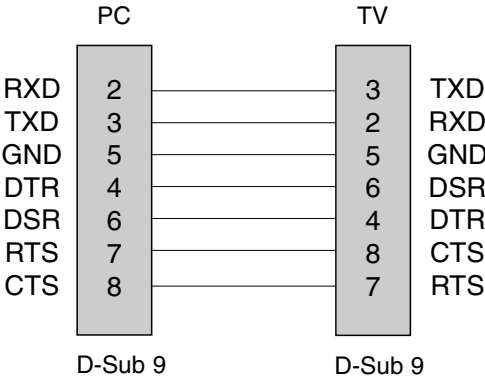
7-Wire Configurations (Serial female-female NULL modem cable)
