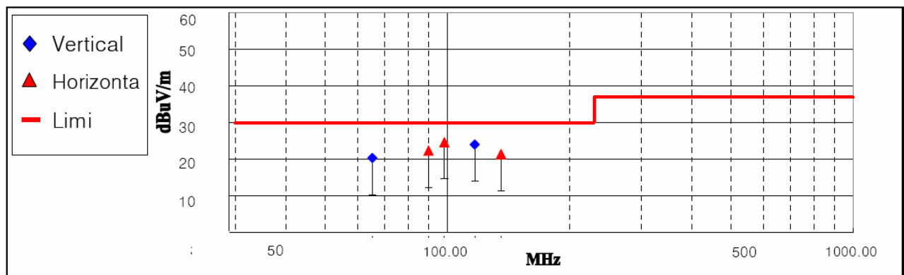
< Fig 4. Radiated emission result _ Analog >
