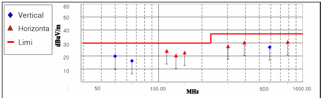
&lt; Fig 5. Radiated emission result _ Digital &gt;
