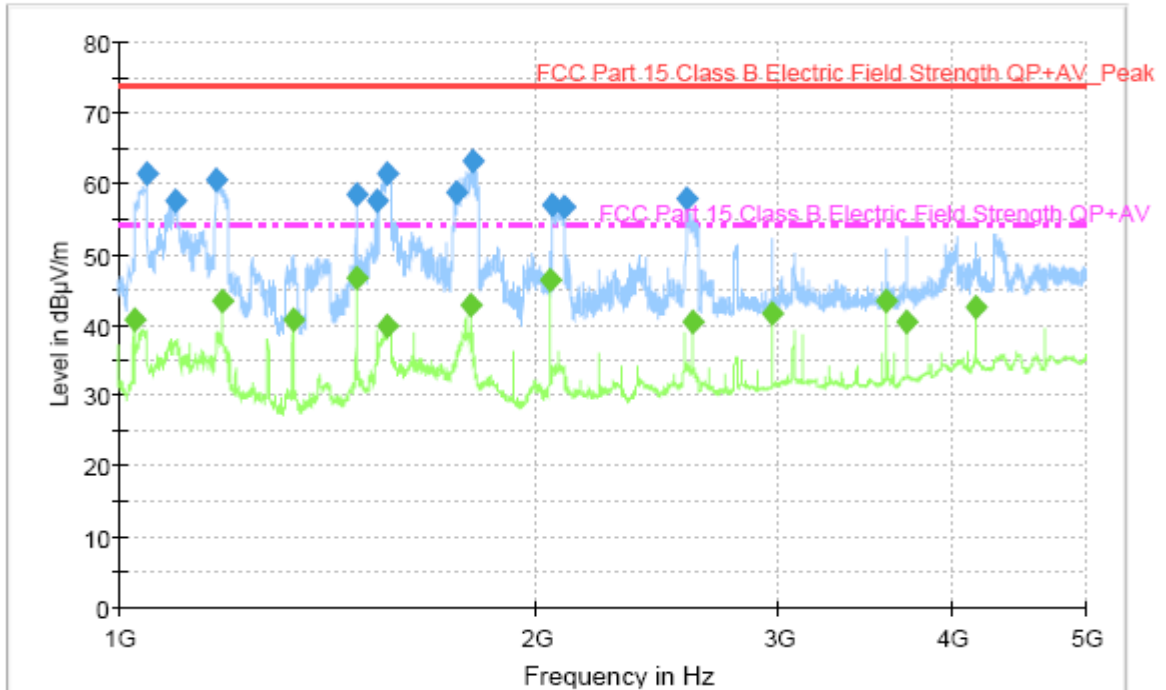
FCC_ESIB_Preamplifier_RE with Scans
