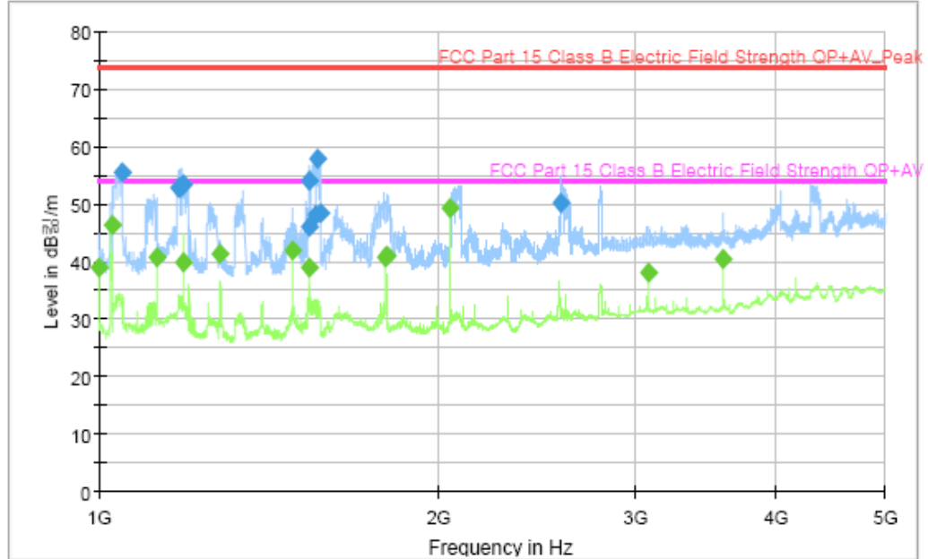
FCC_ESIB_Preamplifier_RE with Scans
