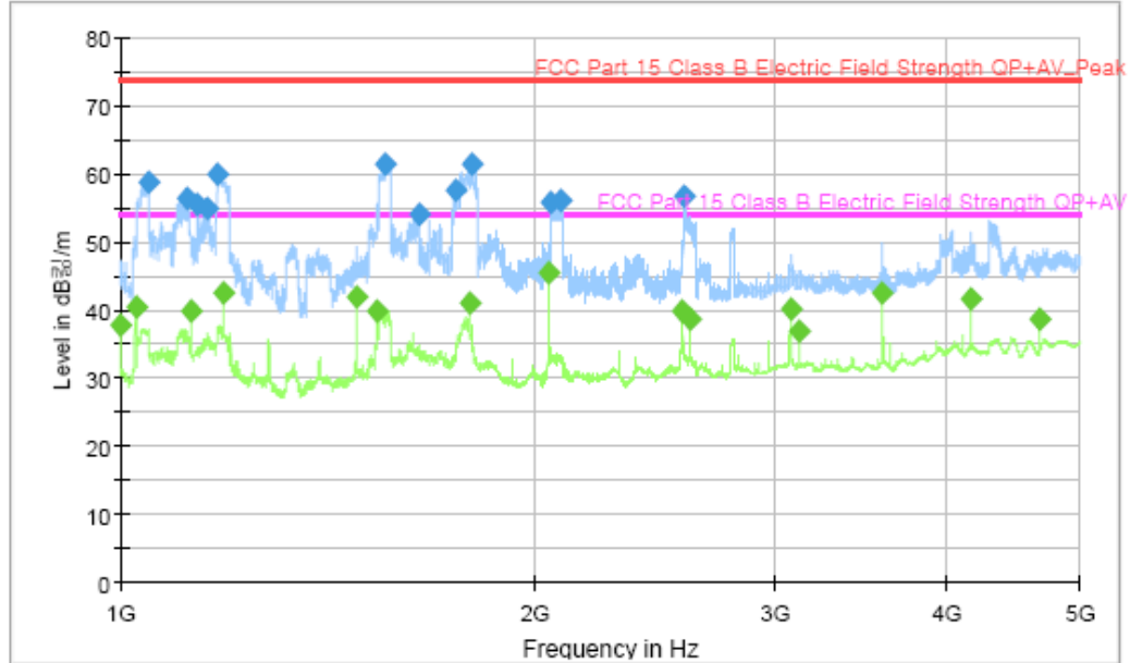
FCC_ESIB_Preamplifier with Scans
