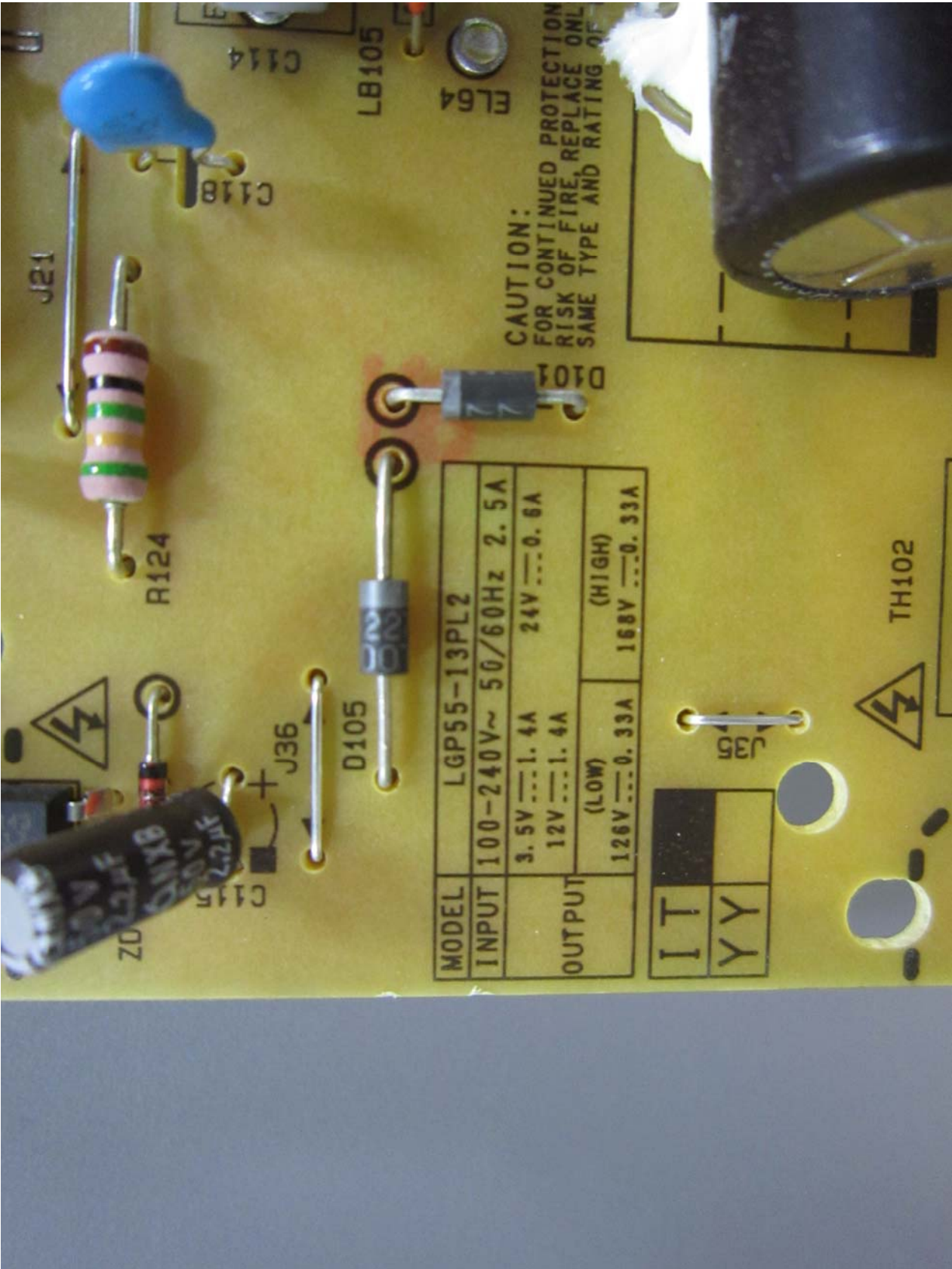
< Power Board Label >
