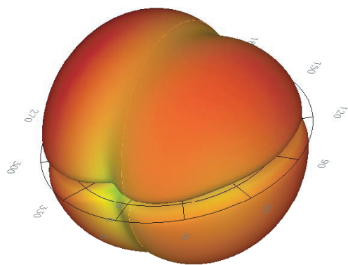
3D Gain Plot
