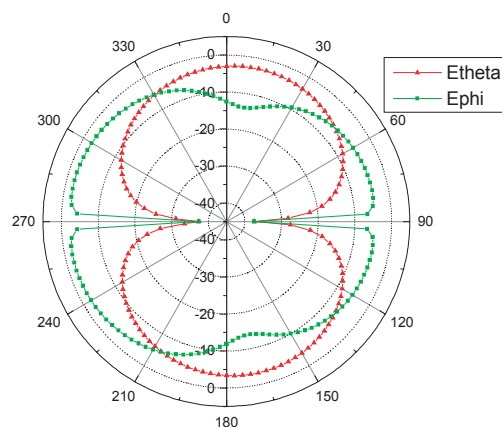
x - z cut (dBi)
