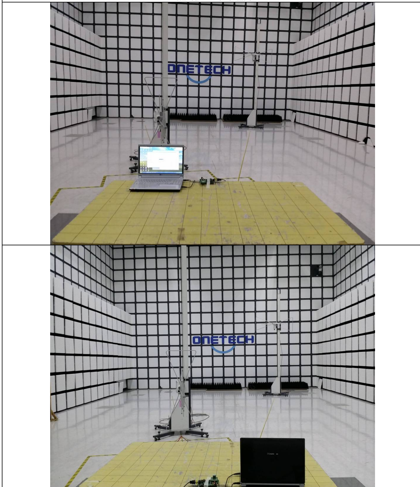
Installed 'X' orientation
