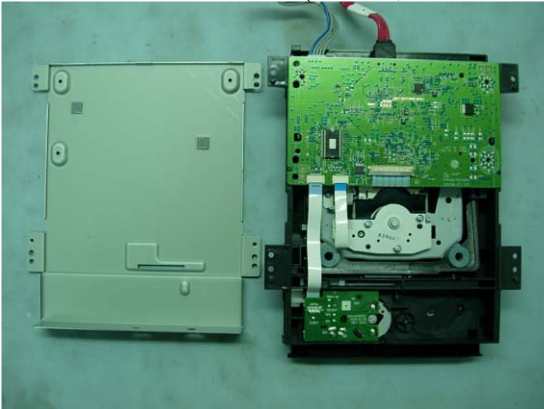
Figure 19 Internal View (DVD Driver, Control Boards/ Back View)
