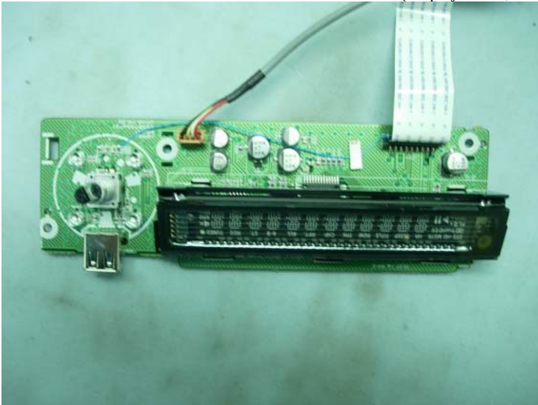
Figure 33 Internal View (Display Board, Front View)
