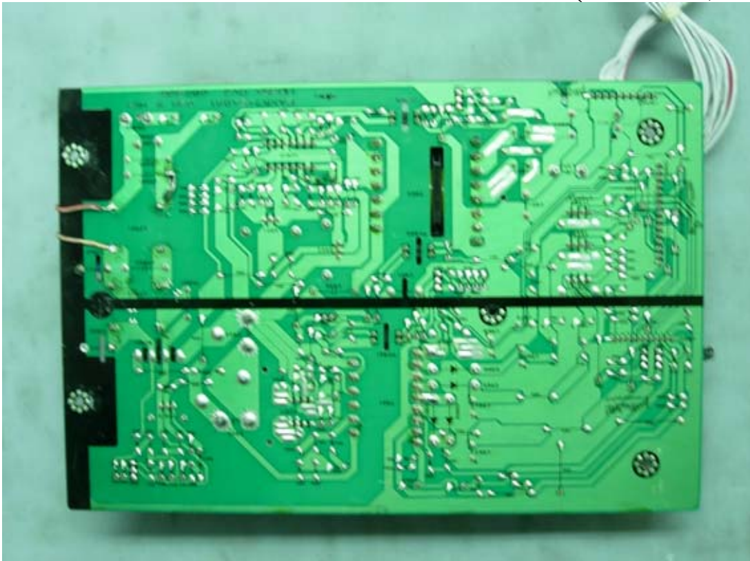
Figure 8 Internal View (Power Board, Back View)
