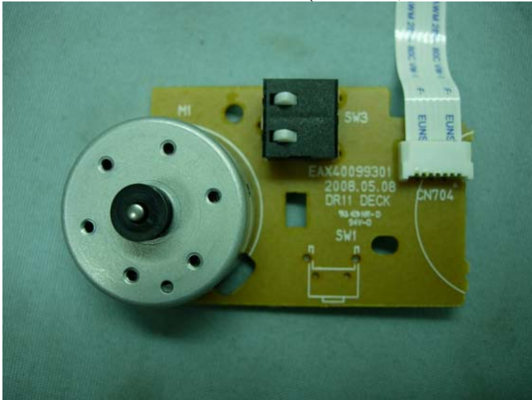
Figure 21 Internal View (DVD Driver, Control Board/Front View)
