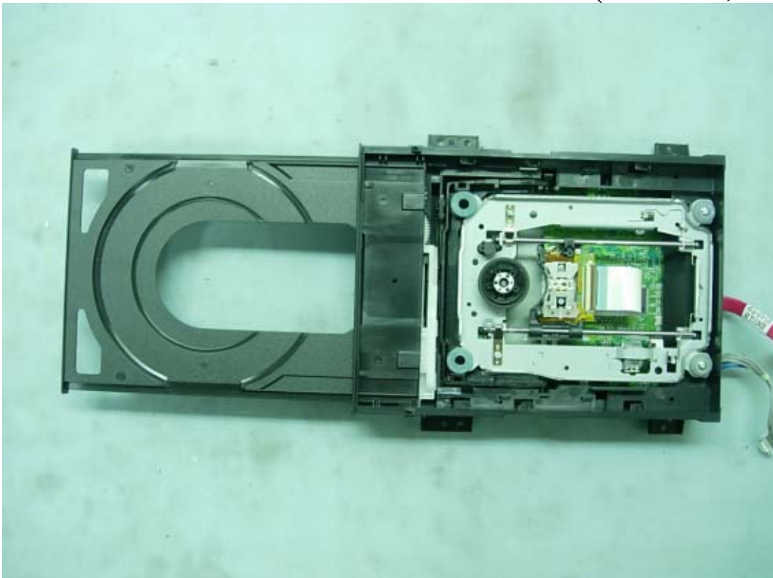
Figure 16 Internal View (DVD Driver, Front View)
