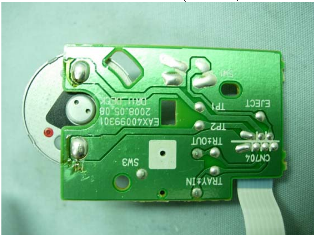
Figure 22 Internal View (DVD Driver, Control Board/Back View)
