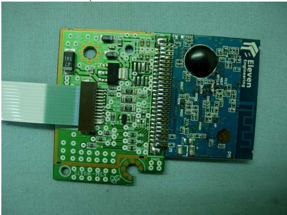
Figure 42 Internal View (RF Module Board/Back View and Control Board/Front View)
