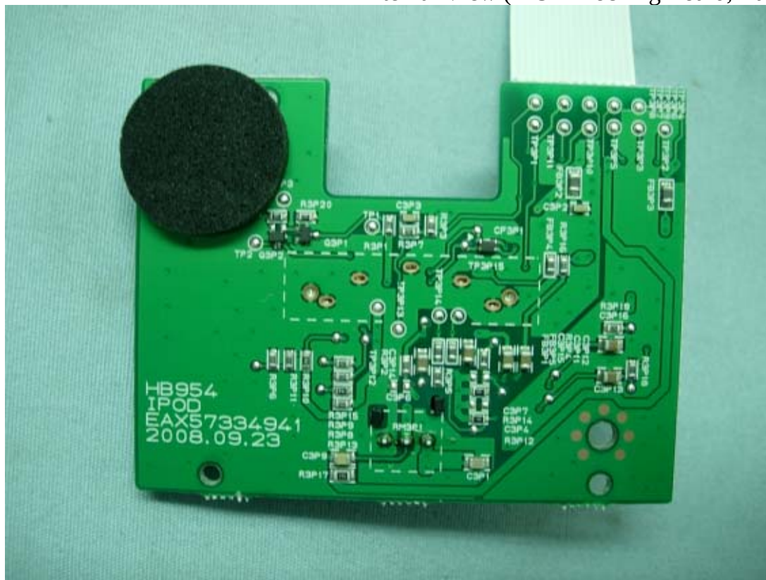
Figure 39 Internal View (IPOD-Docking Board, Back View)
