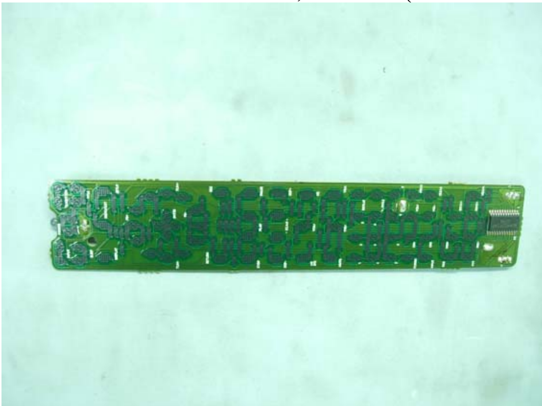
Figure 46 Remote Controller, Internal View (Control Board/ Back View)
