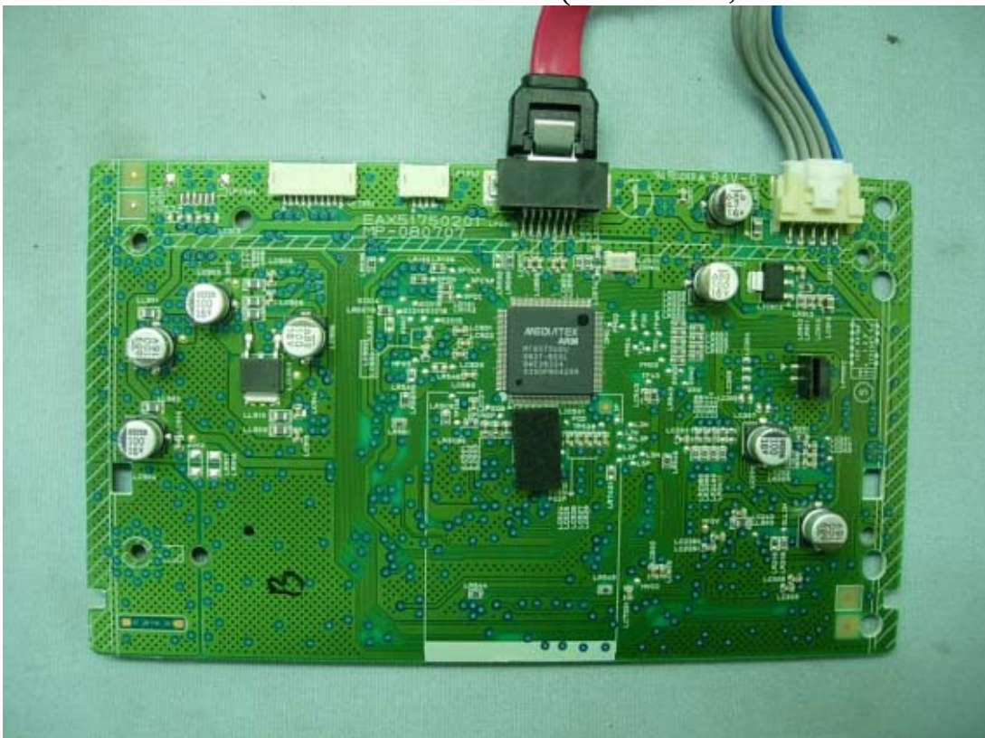
Figure 24 Internal View (DVD Driver, Control Board/ Front View)
