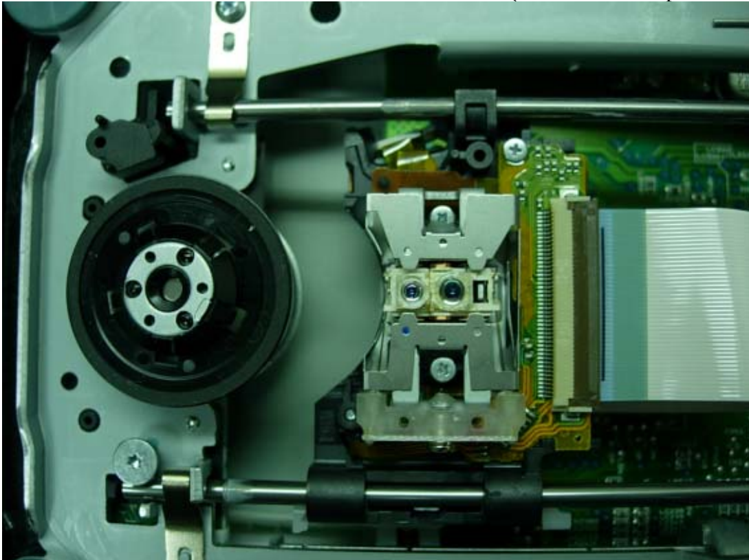
Figure 18 Internal View (DVD Driver, Optical and Motor)
