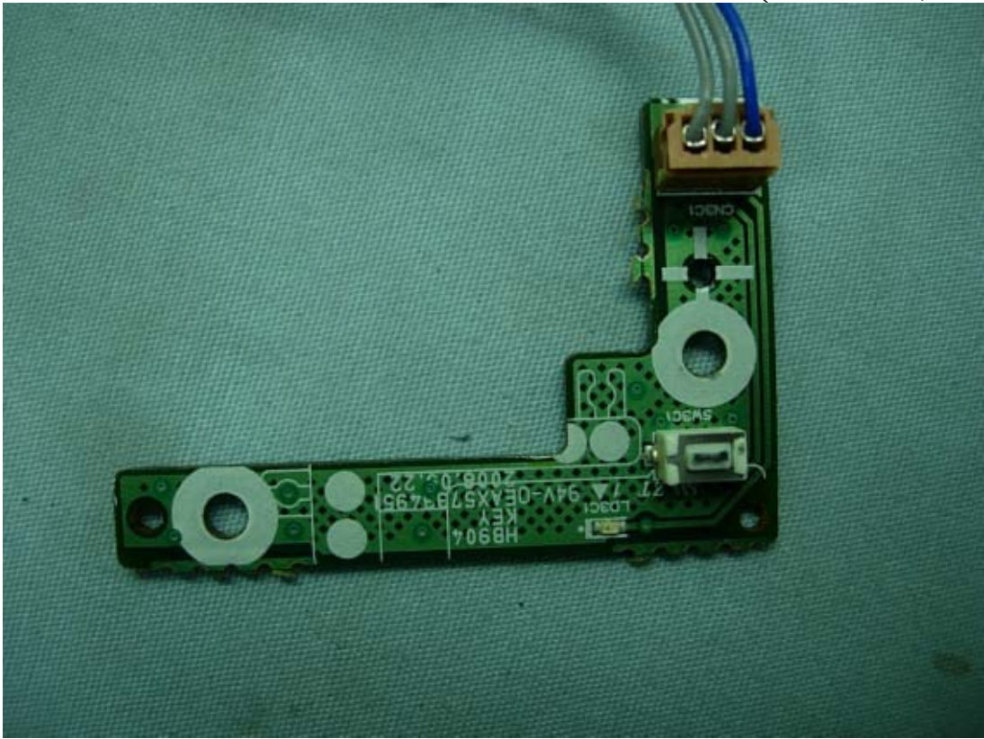
Figure 29 Internal View (Front Board, Front View)
