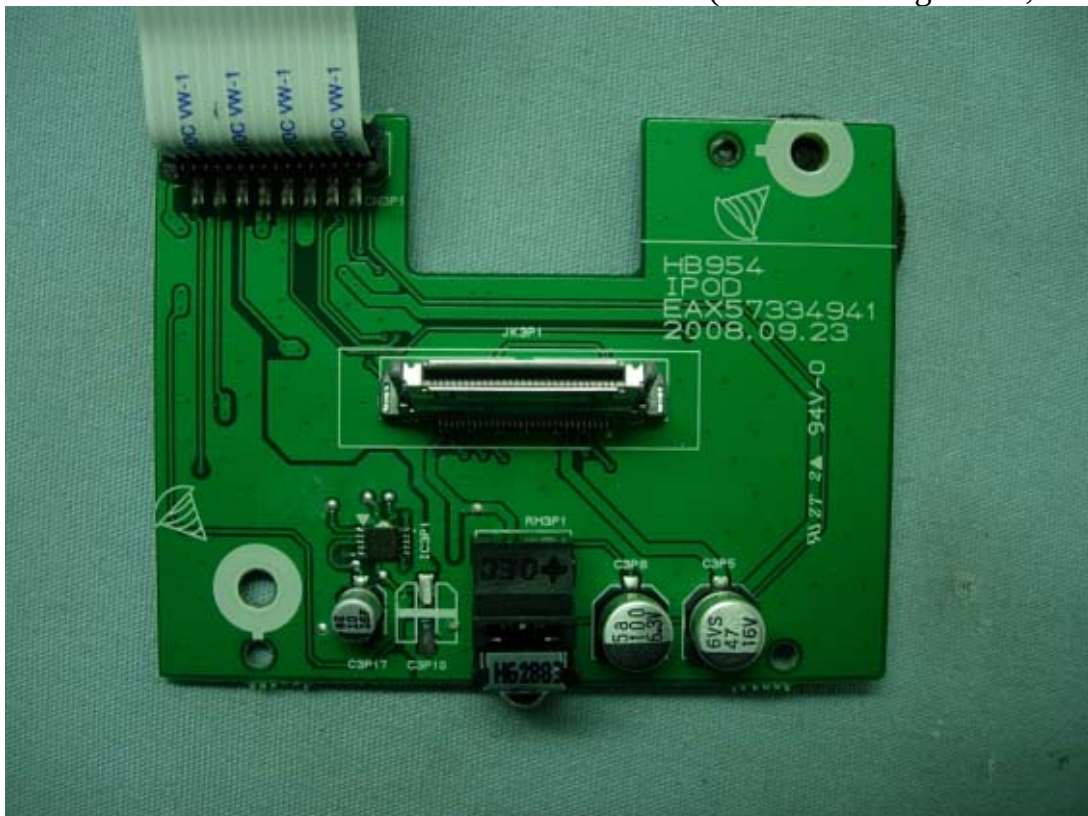
Figure 38 Internal View (IPOD-Docking Board, Front View)
