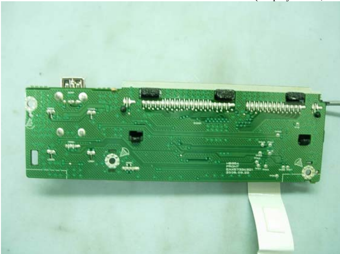
Figure 34 Internal View (Display Board, Back View)
