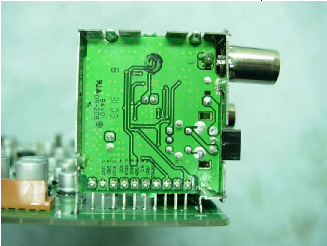
Figure 11 Internal View (Tuner Unit, Back View)
