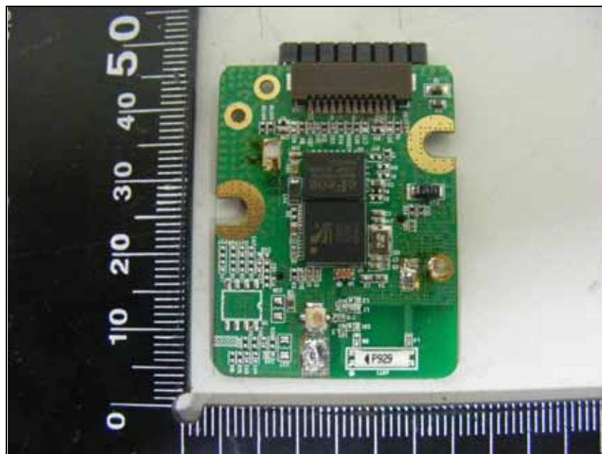
Top view of Main PCB(Removal the shield cap)
