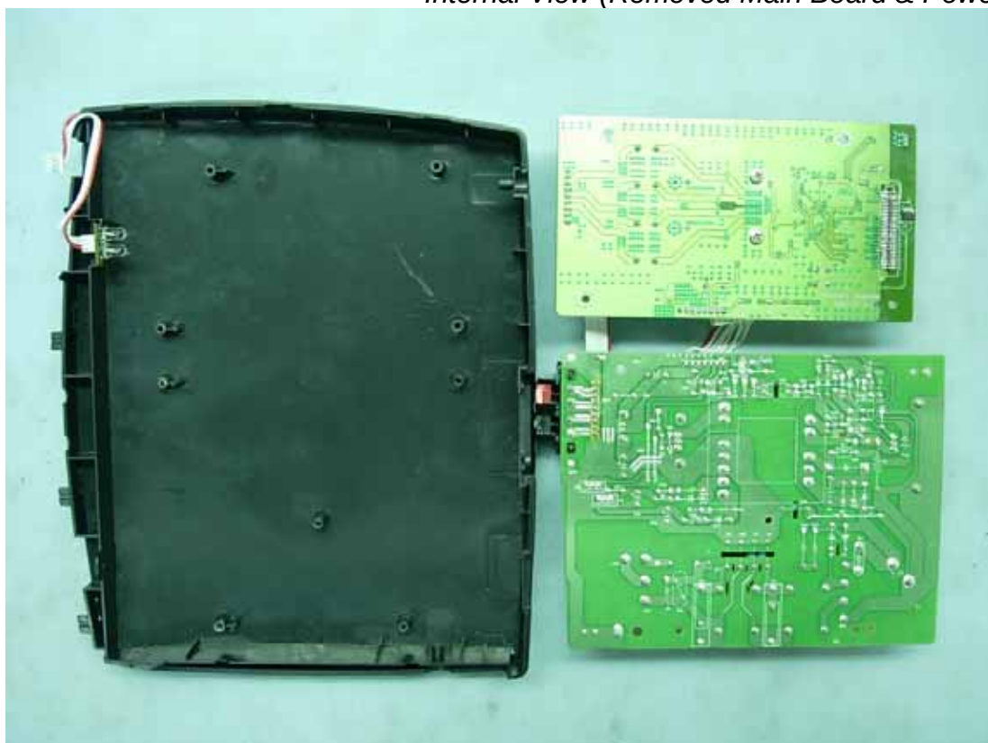
Figure 5 Internal View (Removed Main Board & Power Board)
