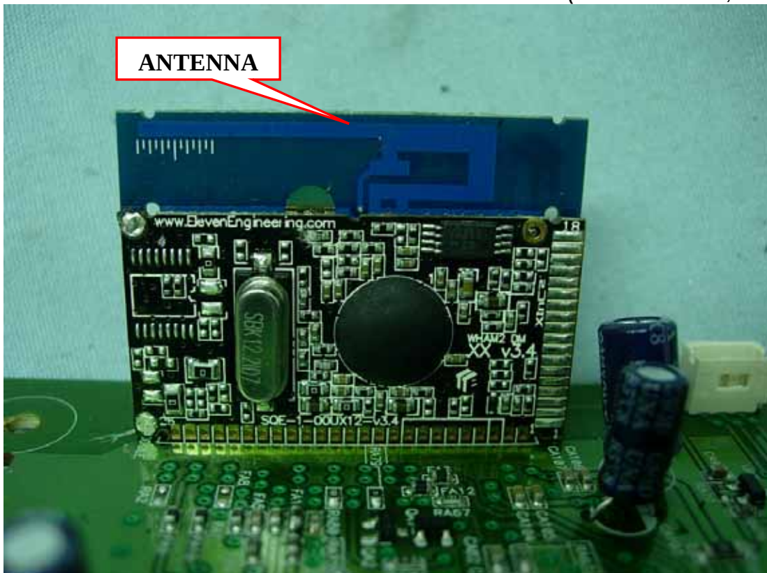
Figure 9 Internal View (TX/RX Module, Back View)
