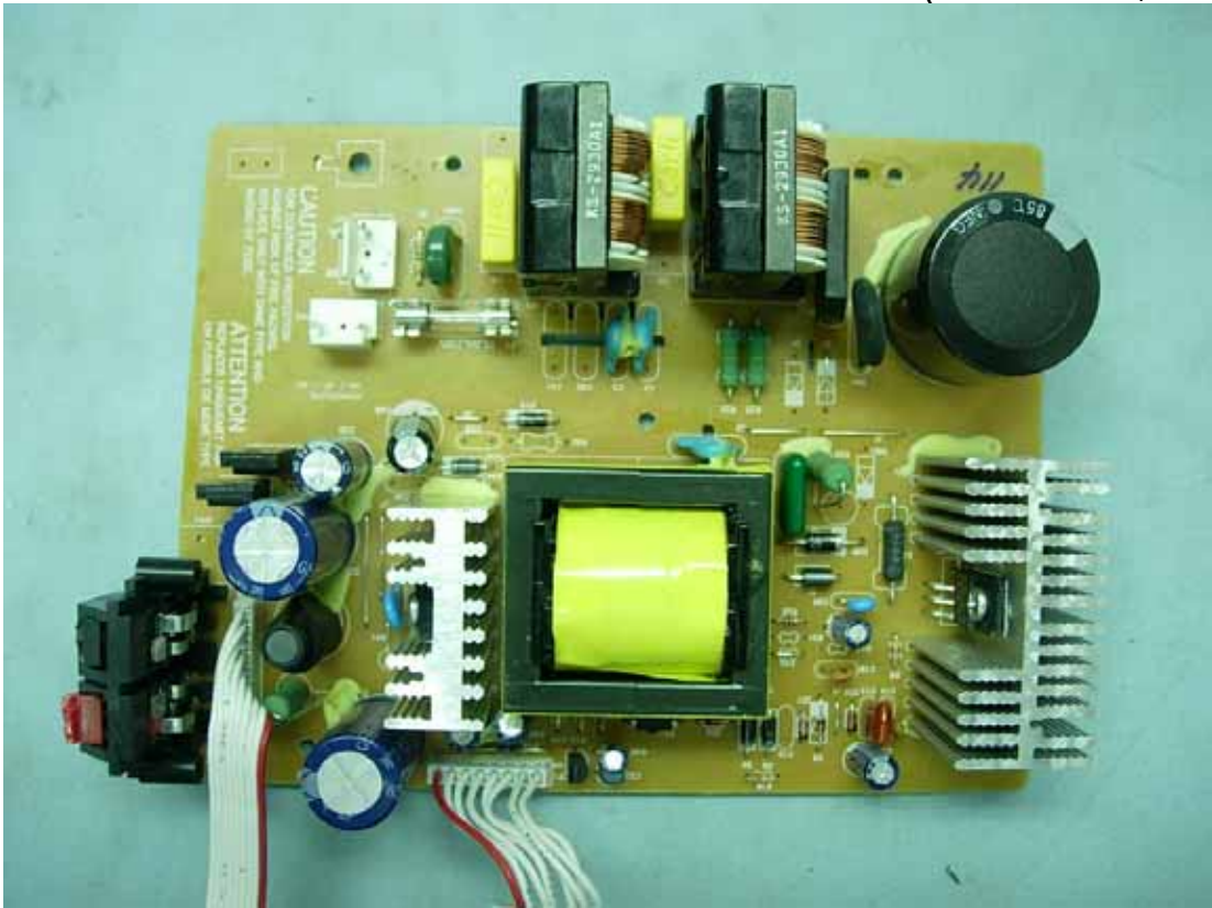
Figure 12 Internal View (Power Board, Front View)
