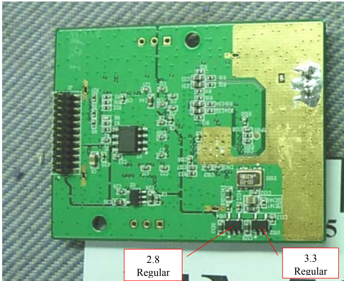
Photo 5 Audio Data Transceiver RF Module, Back View
