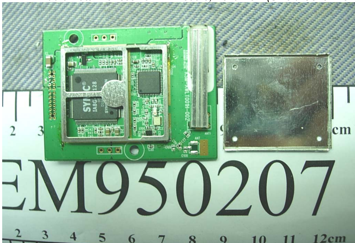
Photos 6 Audio Data Transceiver RF Module, Front View (Shield Cover Removed)
