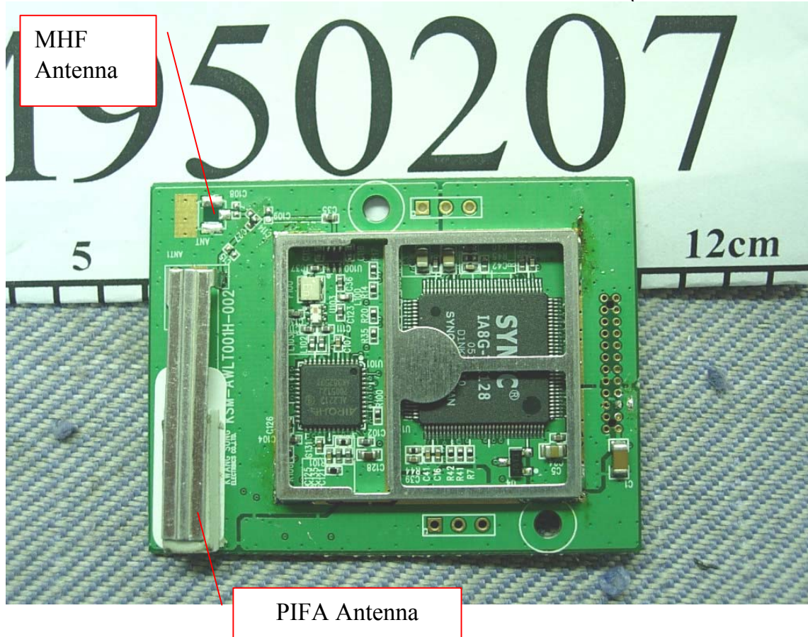
Audio Data Transceiver RF Module, Font View (Without Shield Cover)
