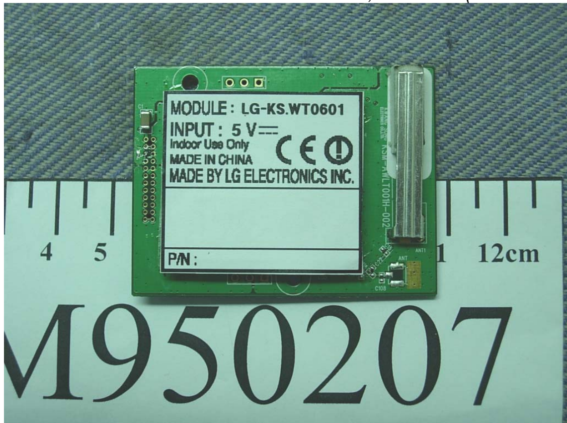
Audio Data Transceiver RF Module, Front View (With Shield Cover)
