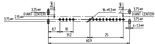
Dimension of P.C.B for Tm-Block Mounting (Viewed from Copper Pattern)
