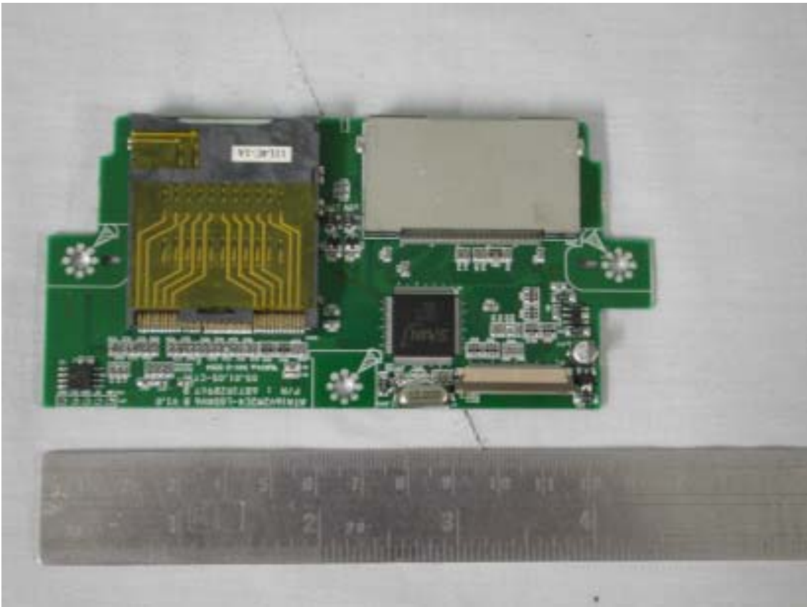
Front Memory Slot PCB
