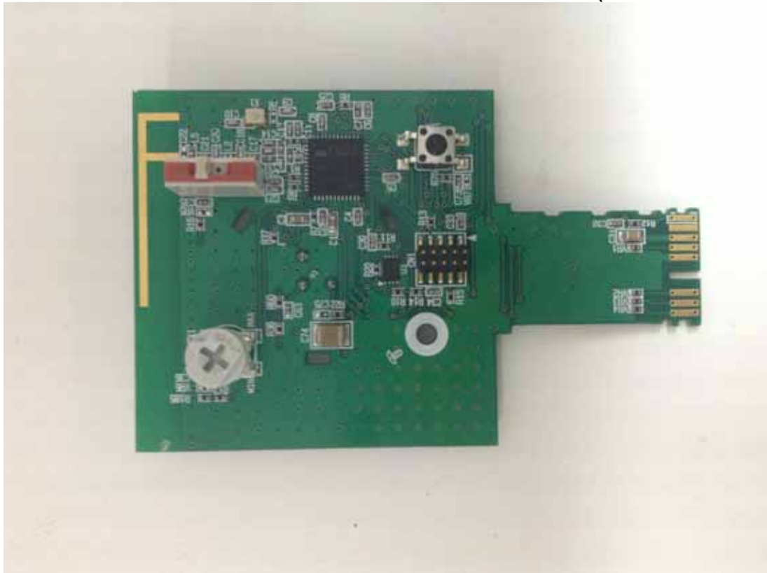
Figure 3 Internal View (Main Board, Front View)
