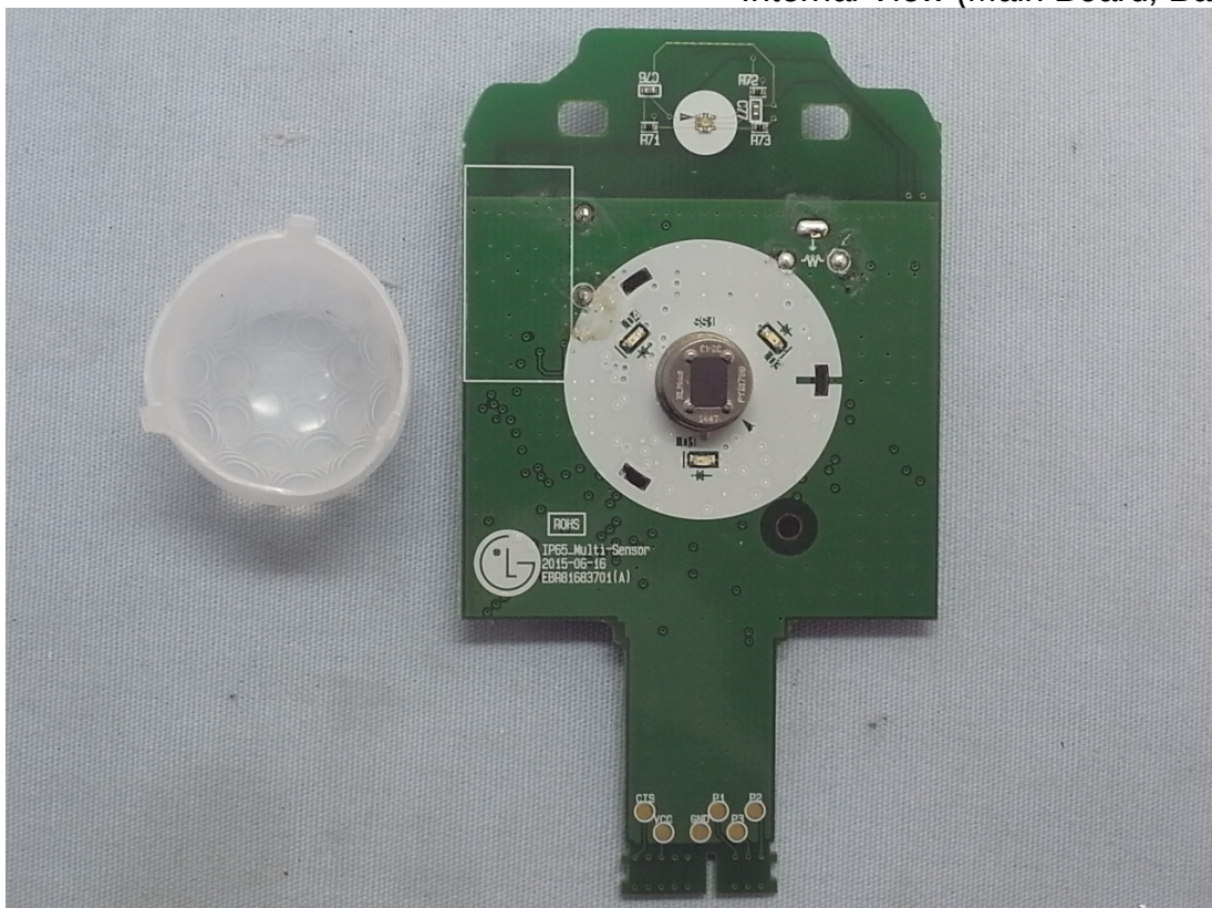
Figure 4 Internal View (Main Board, Back View)
