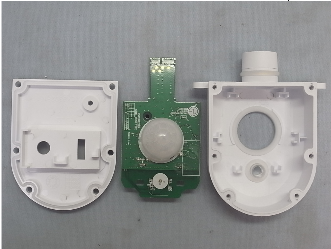
Figure 3 Internal View (Removed Covers)
