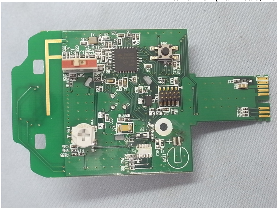
Figure 4 Internal View (Main Board, Front View)
