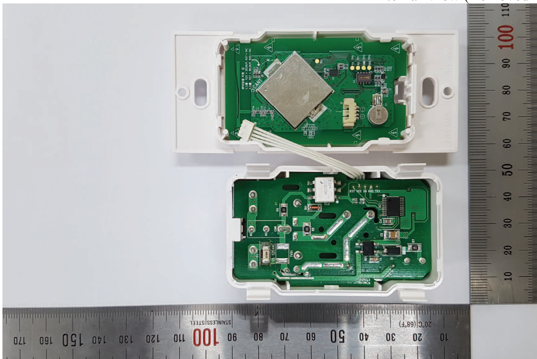
Internal View (Removed Cover)
