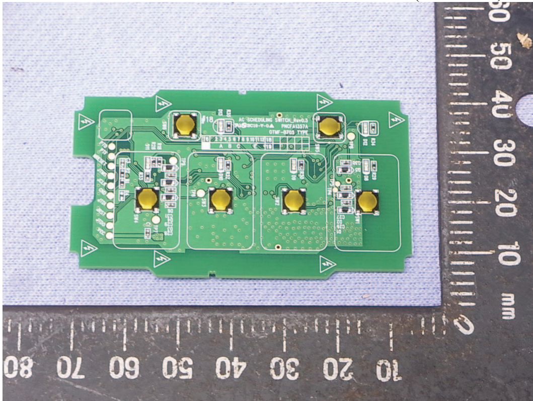
Internal View (Main Board, Back View)
