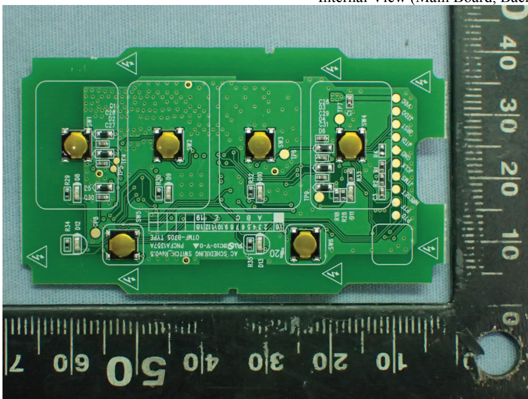
Figure 16 Internal View (Main Board, Back View)
