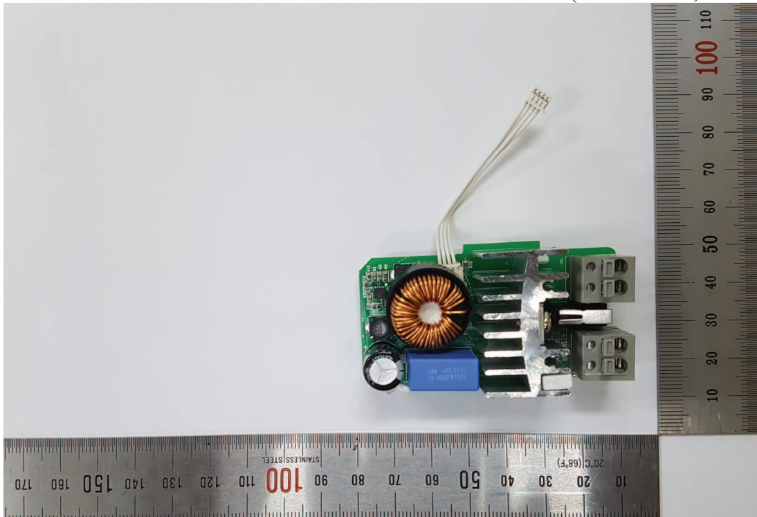
Internal View (Power Board, Front View)
