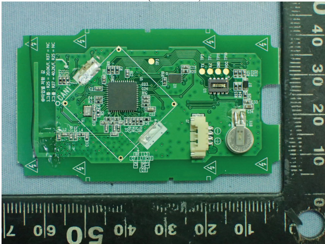
Figure 14 Internal View (Main Board, Front View/Removed Shielded Cover)
