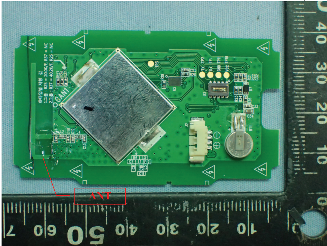
Figure 13 Internal View (Main Board, Front View)
