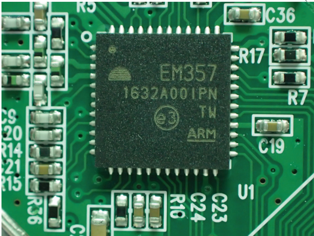
Figure 15 Internal View (RF Chip)
