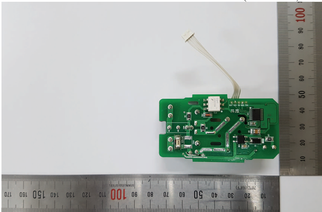
Internal View (Power Board, Back View)
