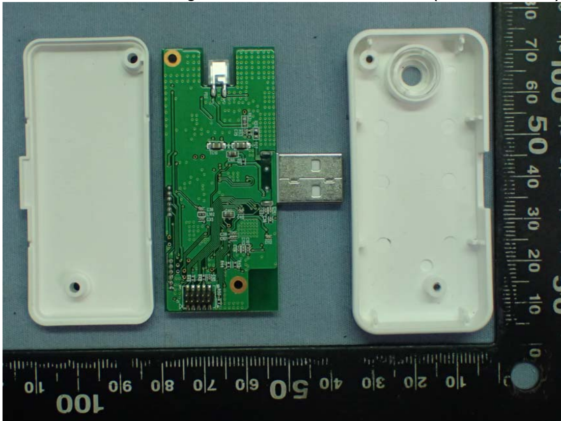
Figure 5 VLC ZigBee Connector, Internal View (Remove Cover)
