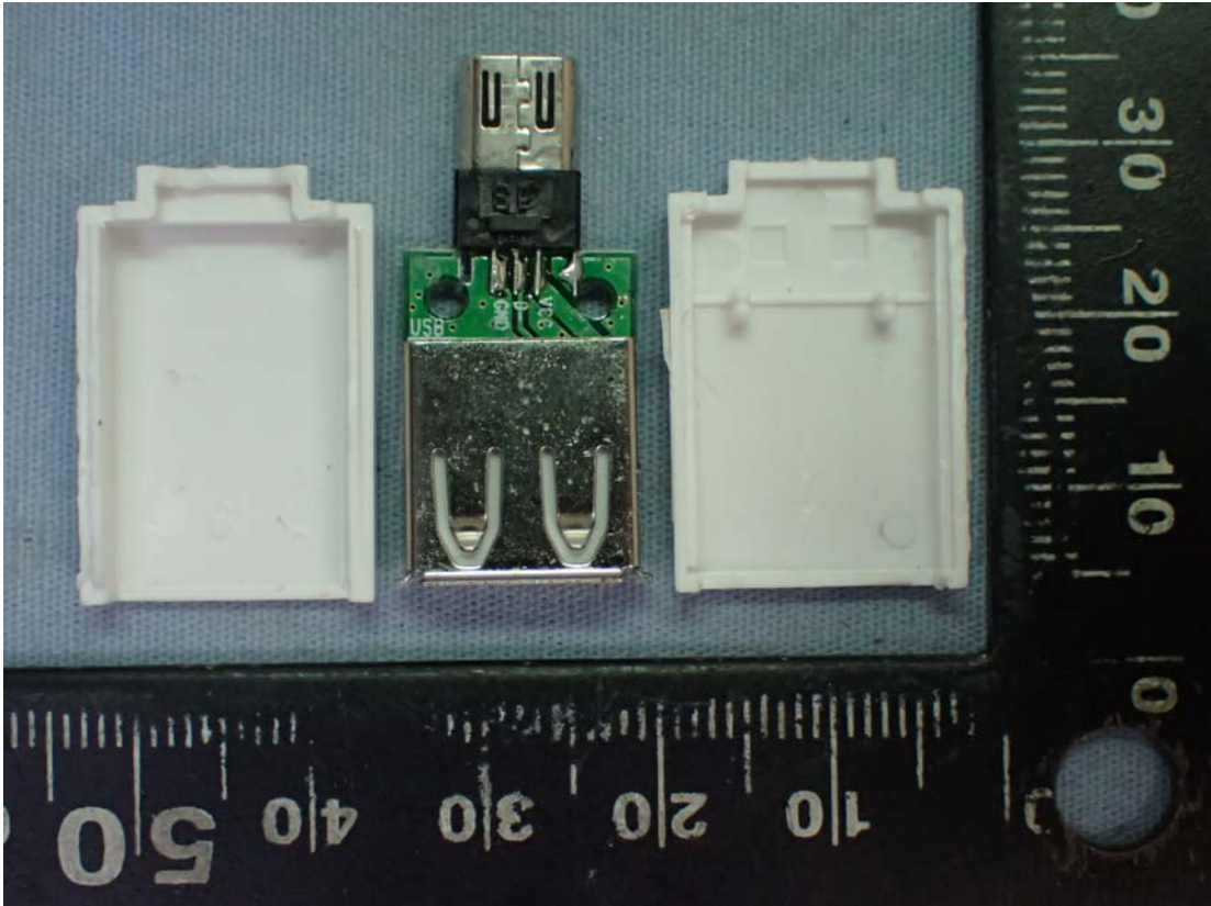
Figure 8 USB OTG, Internal View (Remove Cover)
