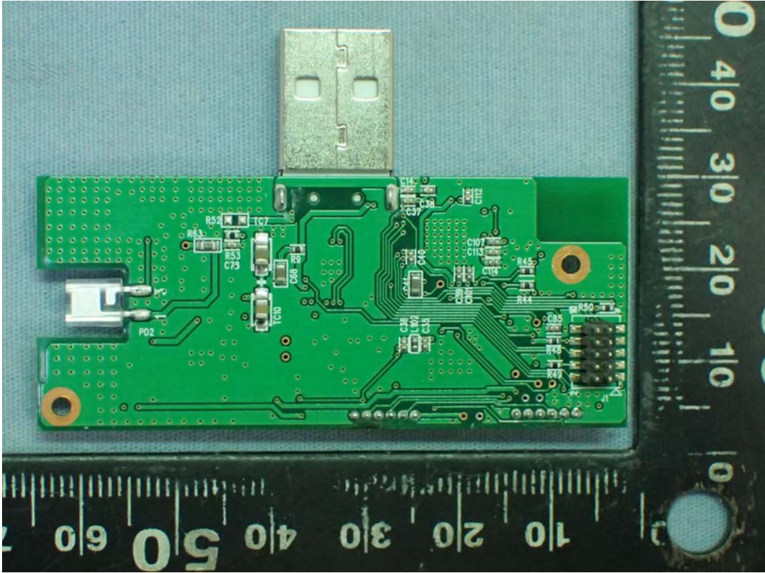
Figure 7 VLC ZigBee Connector, Internal View (Main Board, Back View)
