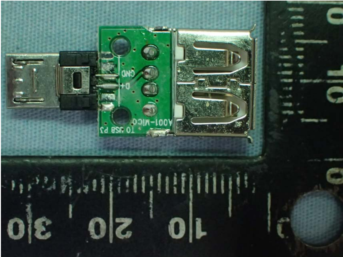
Figure 10 USB OTG, Internal View (Main Board, Back View)
