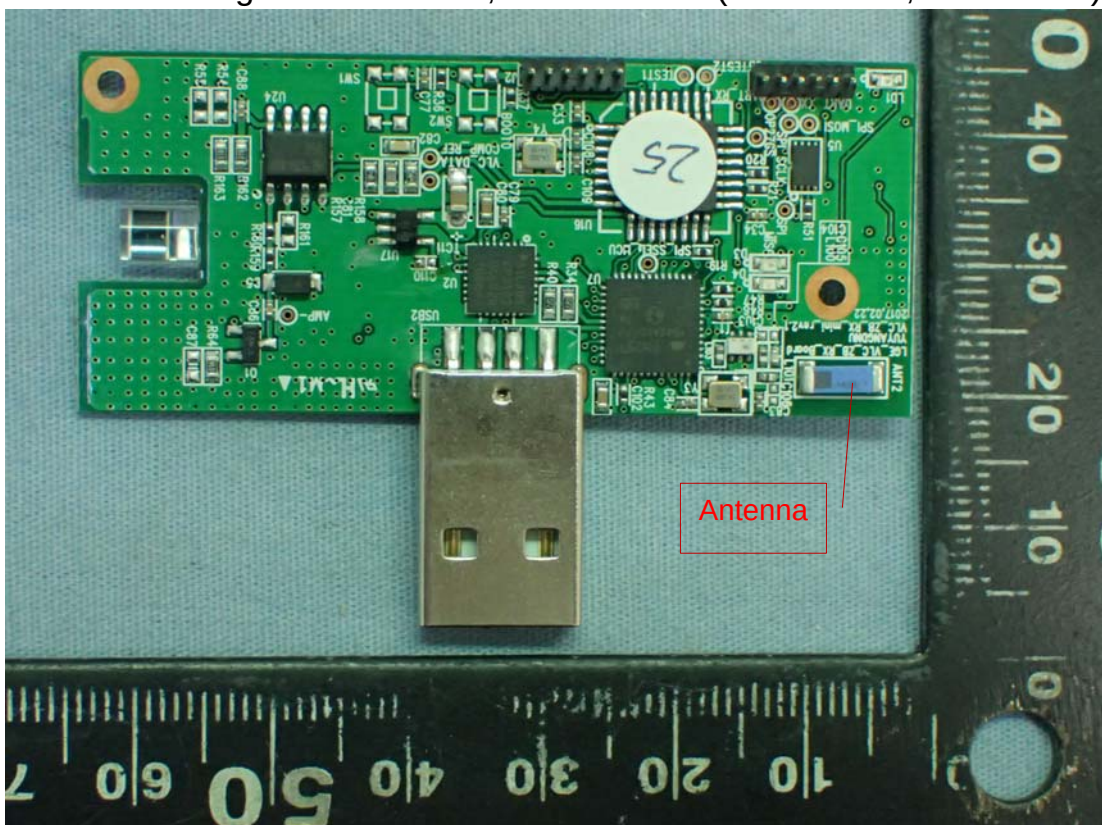
Figure 6 VLC ZigBee Connector, Internal View (Main Board, Front View)
