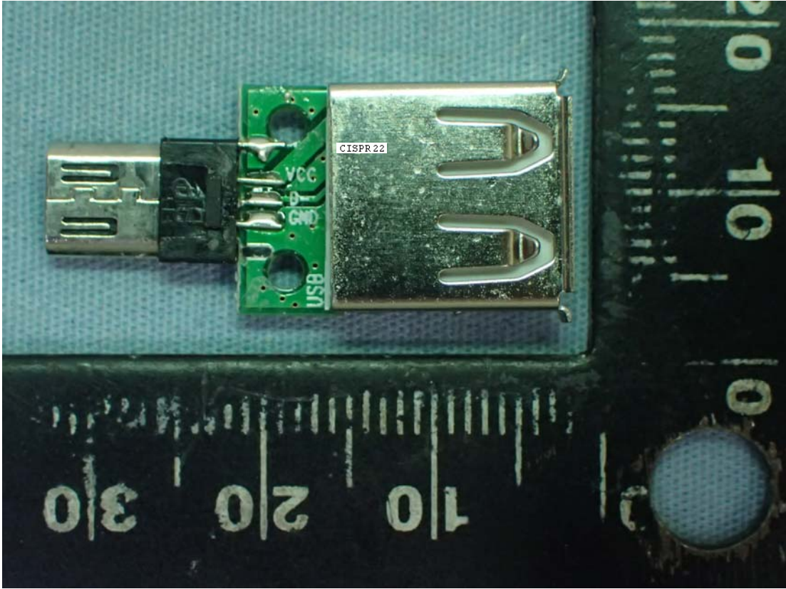
Figure 9 USB OTG, Internal View (Main Board, Front View)
