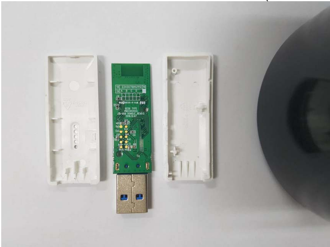
Figure 4 Internal View (Remove Cover)
