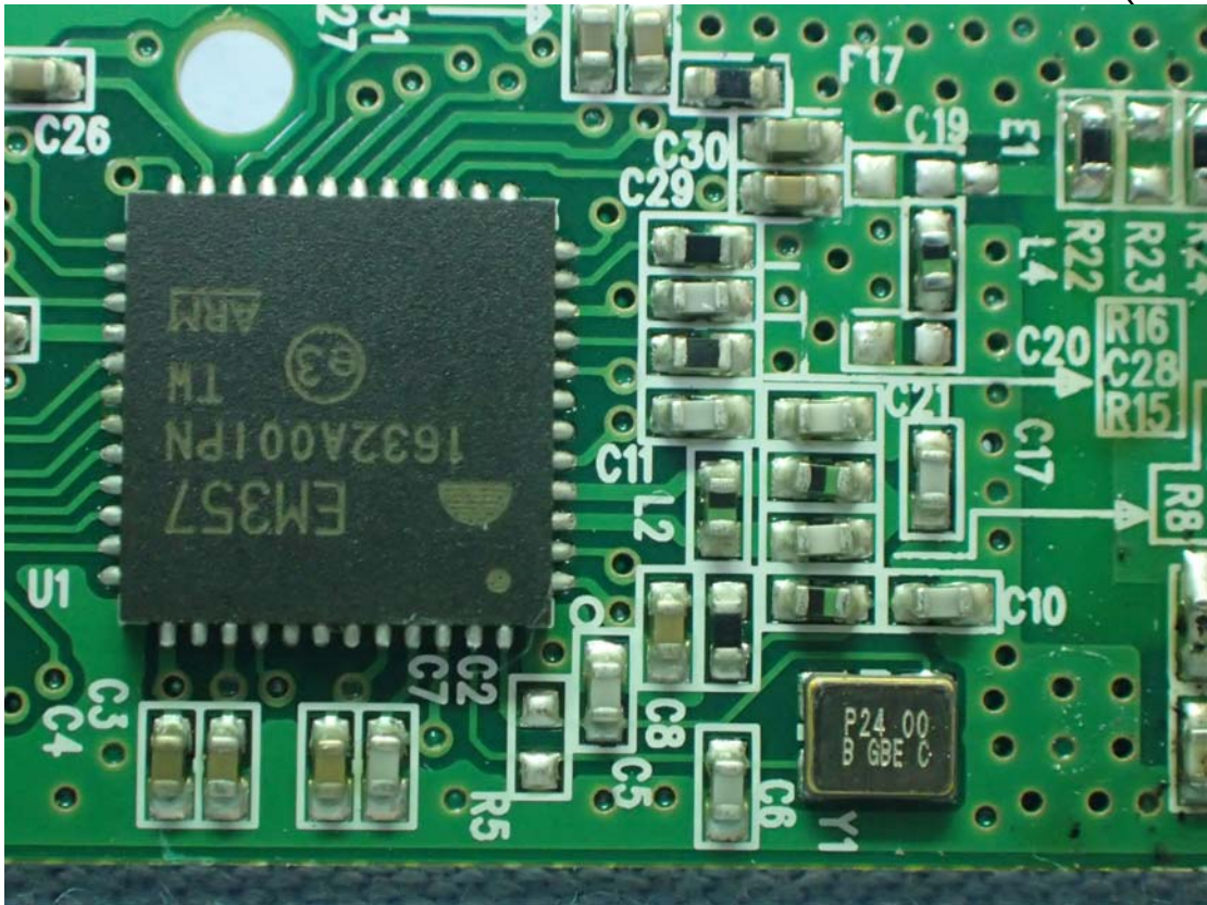
Figure 7 Internal View (RF IC)
