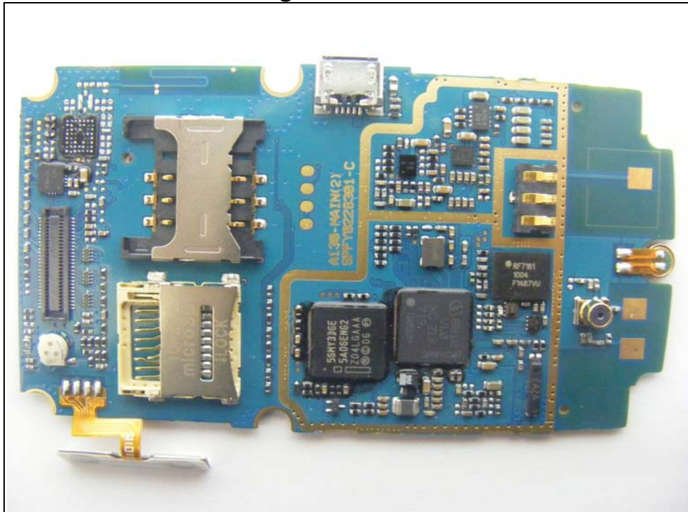
Top view of Main PCB Removing Shield
