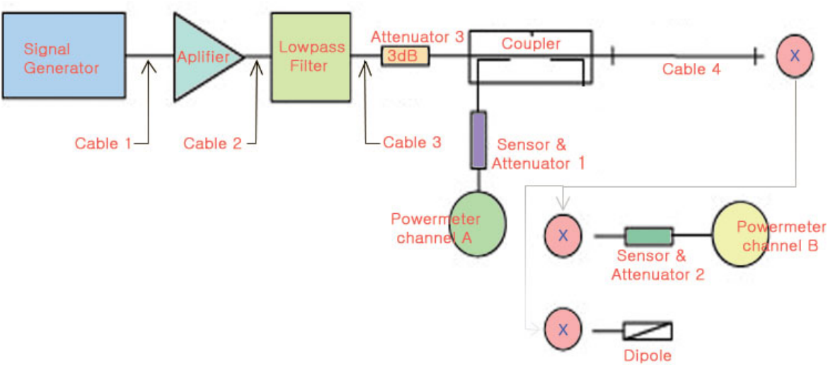
Figure 10.1 Dipole Validation Test Setup
