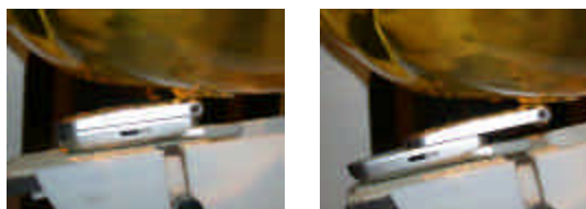
Figure A.4 Left Head SAR Test Setup -- Ear / 15° Tilt Position --
