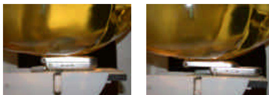
Figure A.5 Right Head SAR Test Setup -- Cheek / Touch Position --
