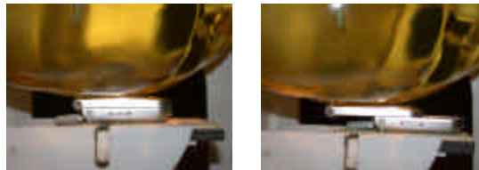
Figure A.1 Right Head SAR Test Setup -- Cheek / Touch Position --
