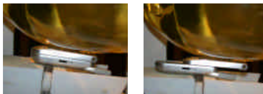
Figure A.3 Left Head SAR Test Setup -- Cheek / Touch Position --
