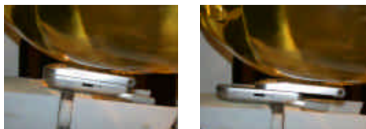
Figure A.7 Left Head SAR Test Setup -- Cheek / Touch Position --
