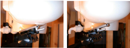
Figure 14.8 Left Head SAR Test Setup -- Ear / Tilt Position --
