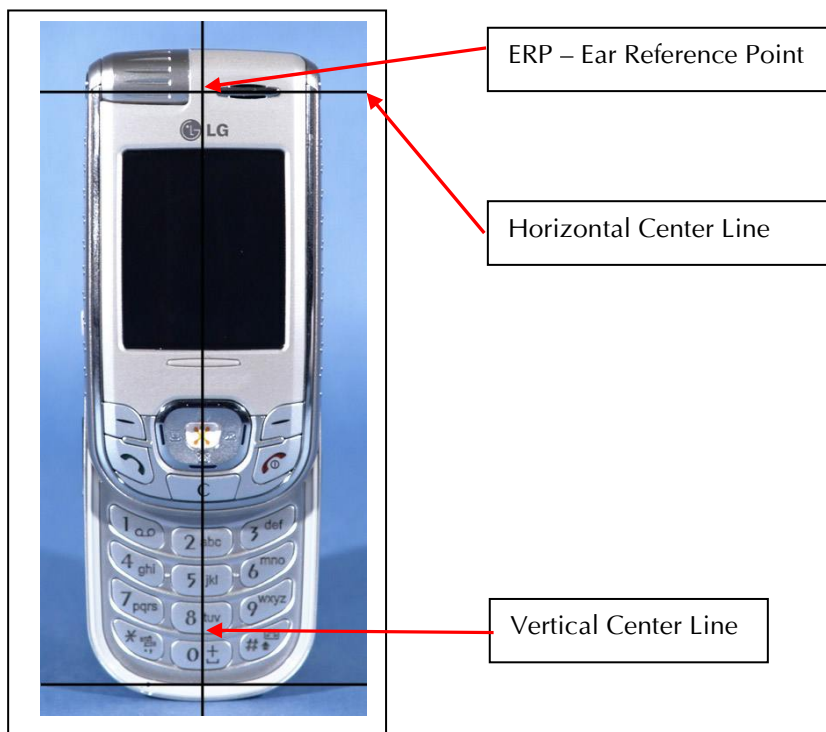
Figure 13.1 Handset Reference Points
