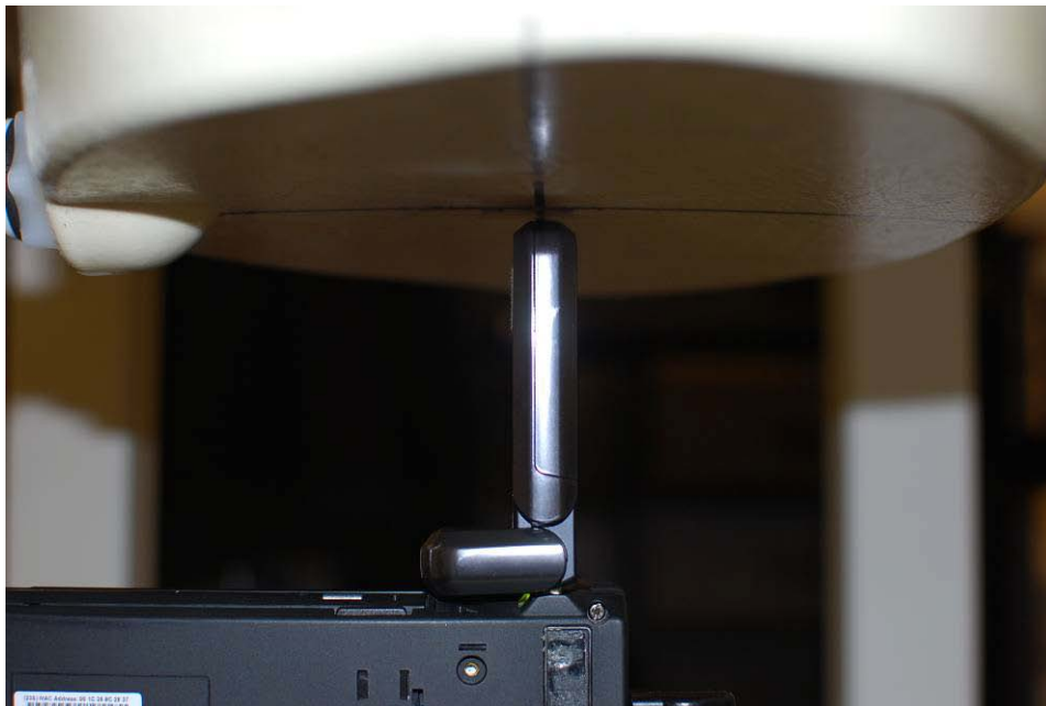
Figure 18-10 SAR Test Setup - Tip
