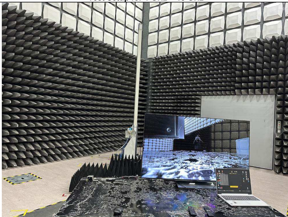
Test Setup for 1 GHz ~ 18 GHz
