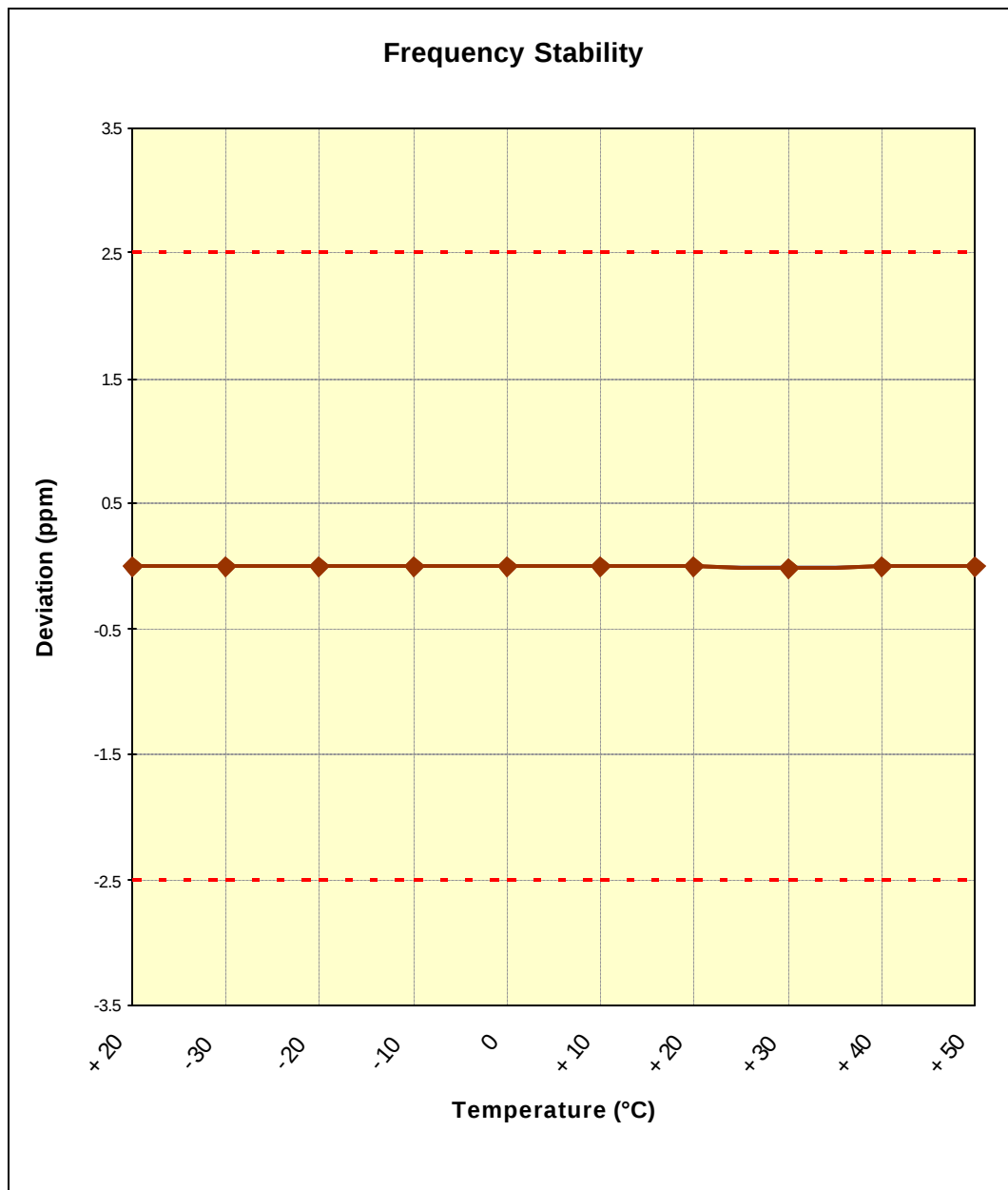
Figure 6-2. Frequency Stability Graph (PCS CDMA Mode – Ch. 600)
