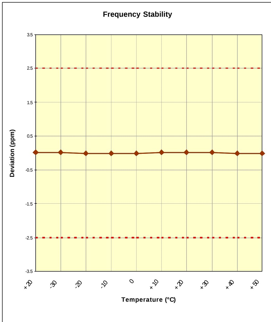
Figure 6-1. Frequency Stability Graph (Cellular CDMA Mode – Ch. 384)
