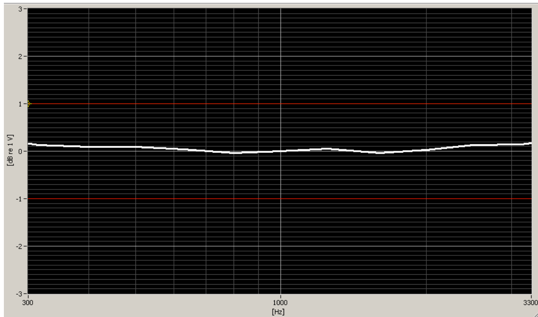
Figure 6-3 Helmholtz Coil Validation for Frequency Response
