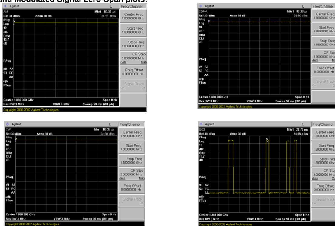
Figure 8-4 Zero-Span Plots
