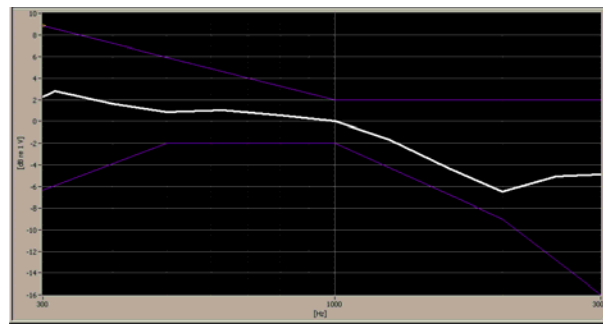
Figure 6-1 Axial Frequency Response
