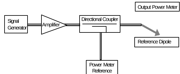
Figure 7-3 Setup to Dipole
