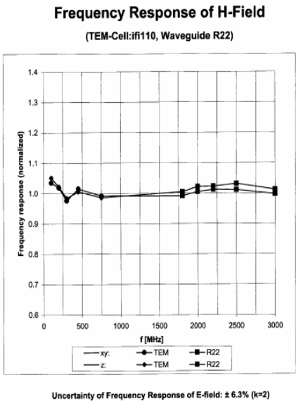
Figure 5-4 H-Field Probe Frequency Response
