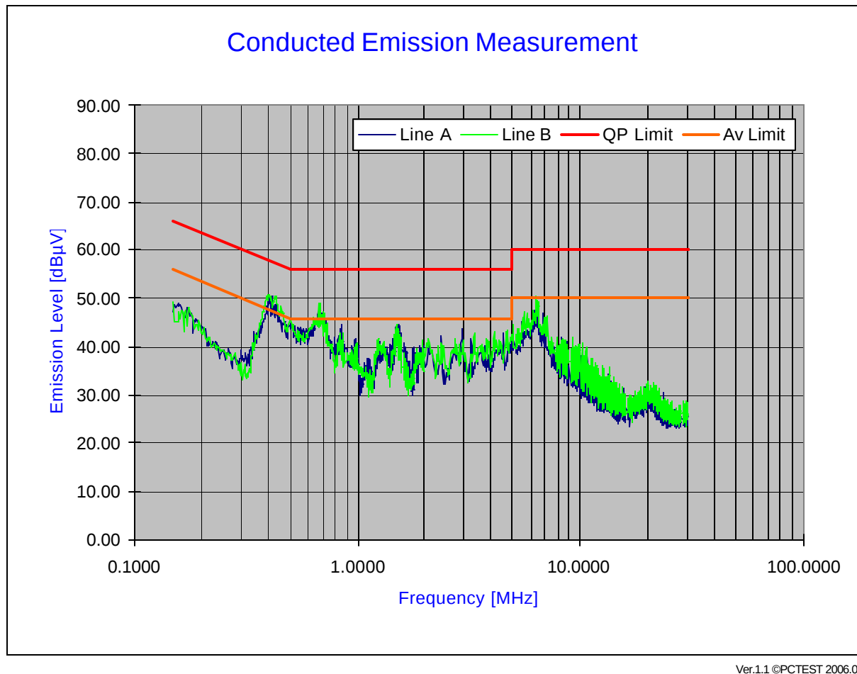
Plot 6-18. Line Conducted Plot with Bluetooth
