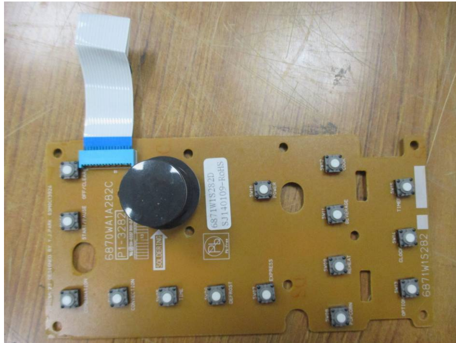
<PCB – Top of Control board>
