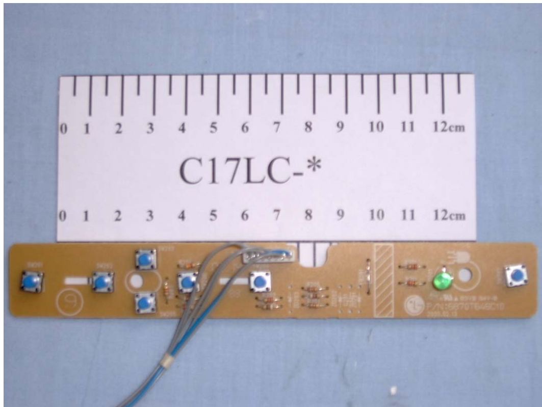
FIGURE 8 COLOR MONITOR (M/N:C17LC-*) CONTROL PANEL BOARD (COMPONENT SIDE)
