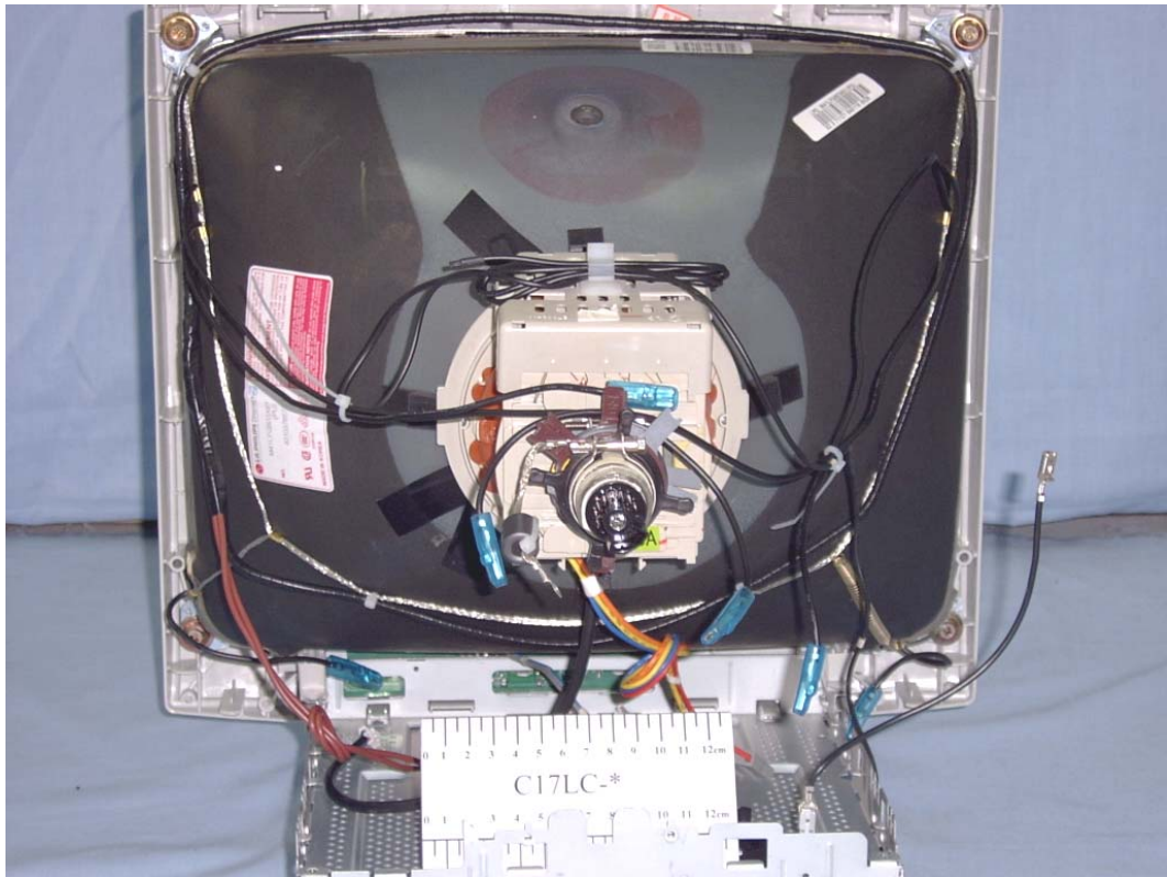
FIGURE 3 COLOR MONITOR (M/N:C17LC-*) CRT TUBE
