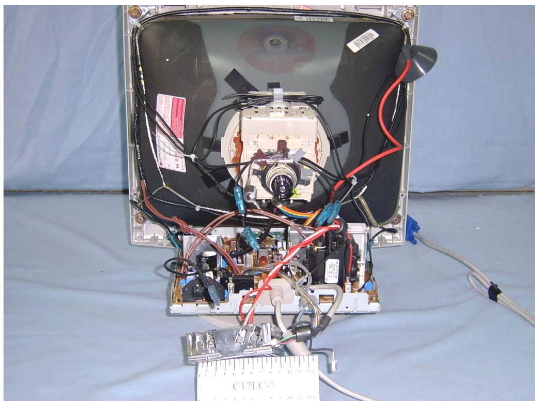
FIGURE 2 COLOR MONITOR (M/N:C17LC-*) COVER REMOVED 2
