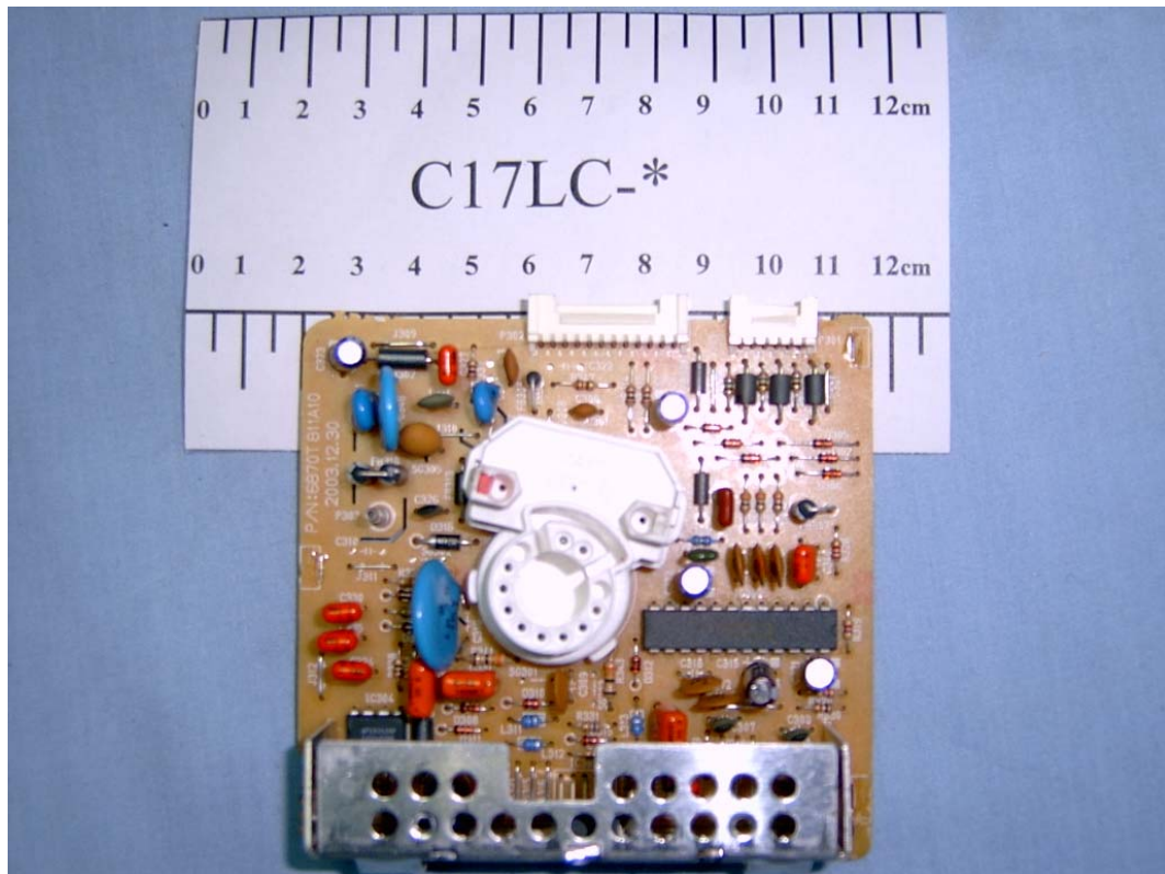
FIGURE 6 COLOR MONITOR (M/N:C17LC-*) CRT BOARD (COMPONENT SIDE)
