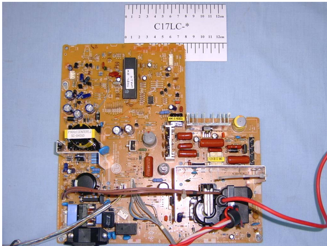
FIGURE 4 COLOR MONITOR (M/N:C17LC-*) MAIN BOARD (COMPONENT SIDE)
