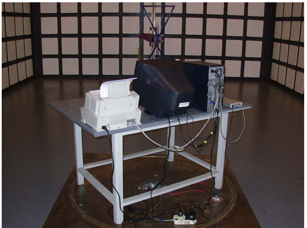
SETUP WITH MAXIMUM DETECTED EMISSION AT VERTICAL POLARIZATION (VGA 1280*1024@60Hz)
