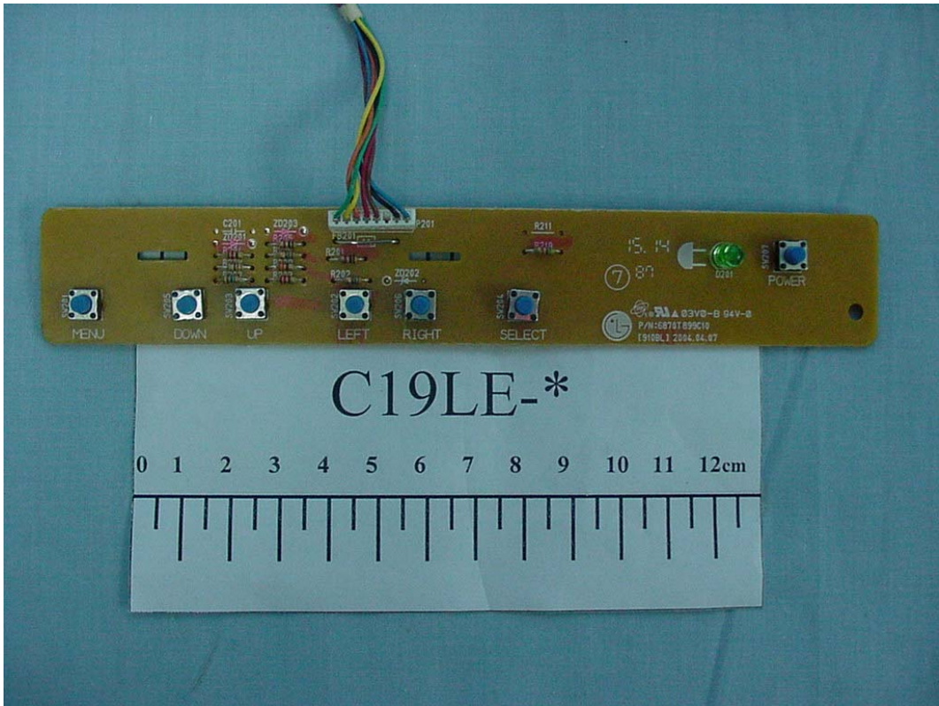
FIGURE 9 COLOR MONITOR (M/N: C19LE-*) CONTROL PANEL BOARD (COMPONENT SIDE)
