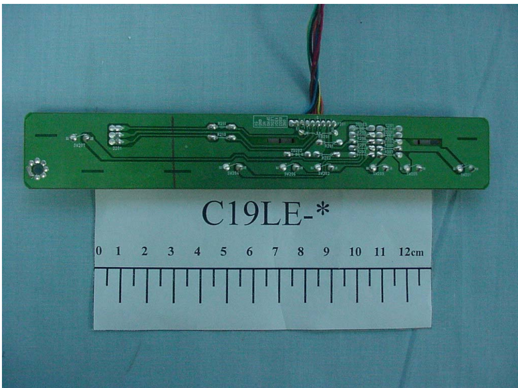
FIGURE 10 COLOR MONITOR (M/N:C19LE-*) CONTROL PANEL BOARD (SOLDERED SIDE)
