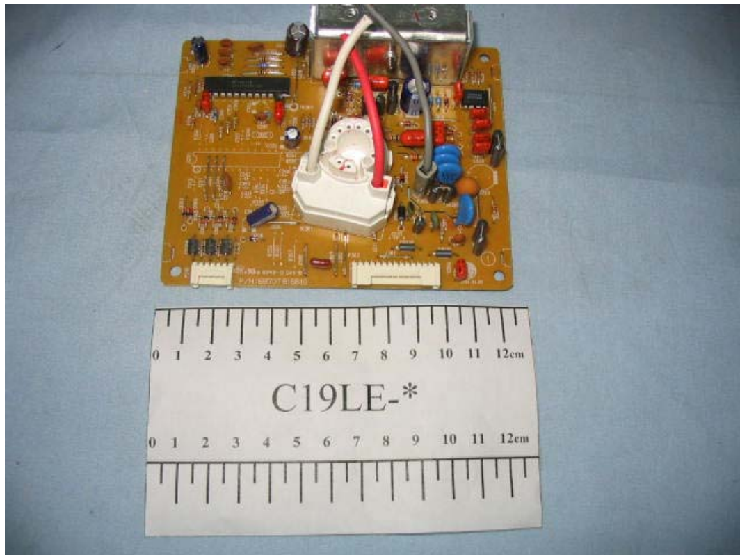
FIGURE 7 COLOR MONITOR (M/N: C19LE-*) CRT BOARD (COMPONENT SIDE)
