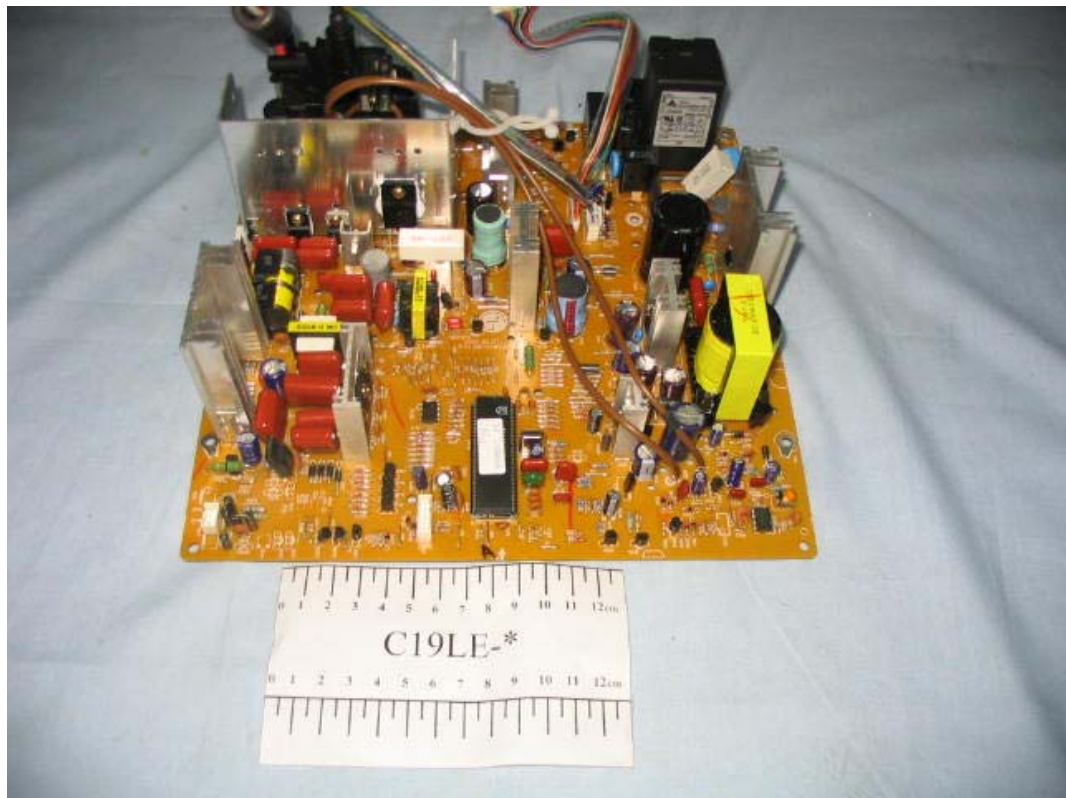
FIGURE 5 COLOR MONITOR (M/N:C19LE-*) MAIN BOARD (COMPONENT SIDE)
