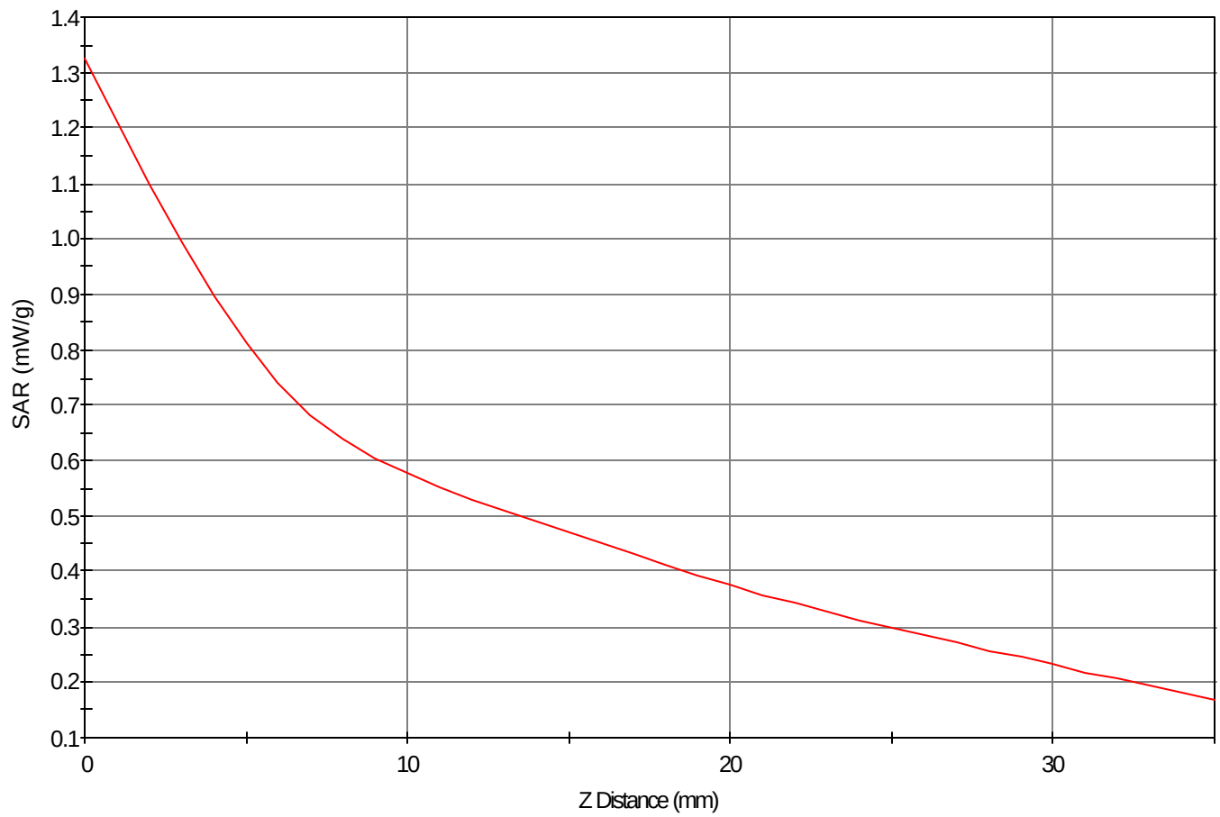
SAR - Z Axis at Hotspot x:77.0 y:19.0
