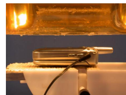
Figure A.9 Body SAR Test Setup -- w/o Belt Clip --
