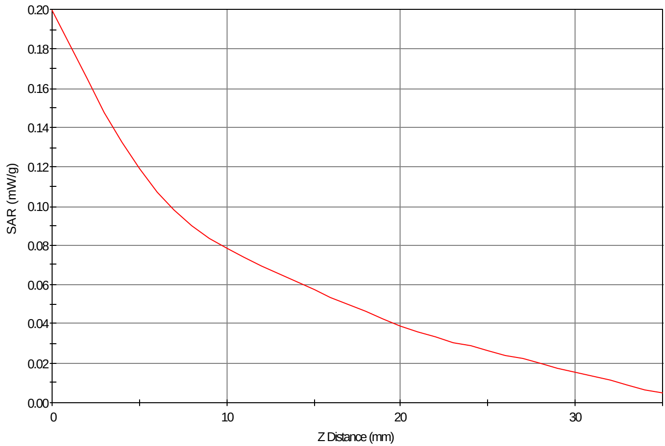
SAR - Z Axis at Hotspot x:89.0 y:-9.0
