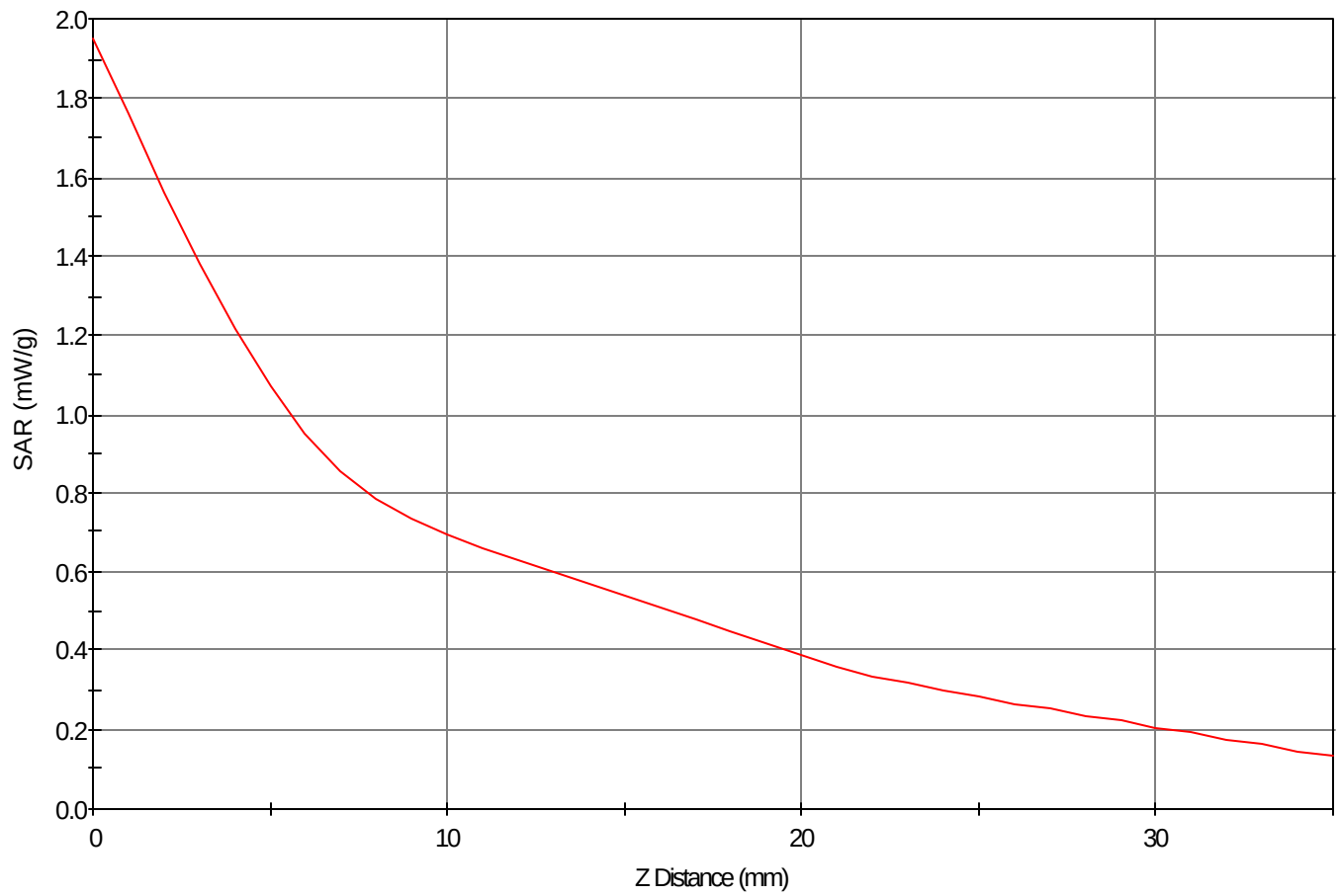
SAR - Z Axis at Hotspot x:-7.0 y:38.0
