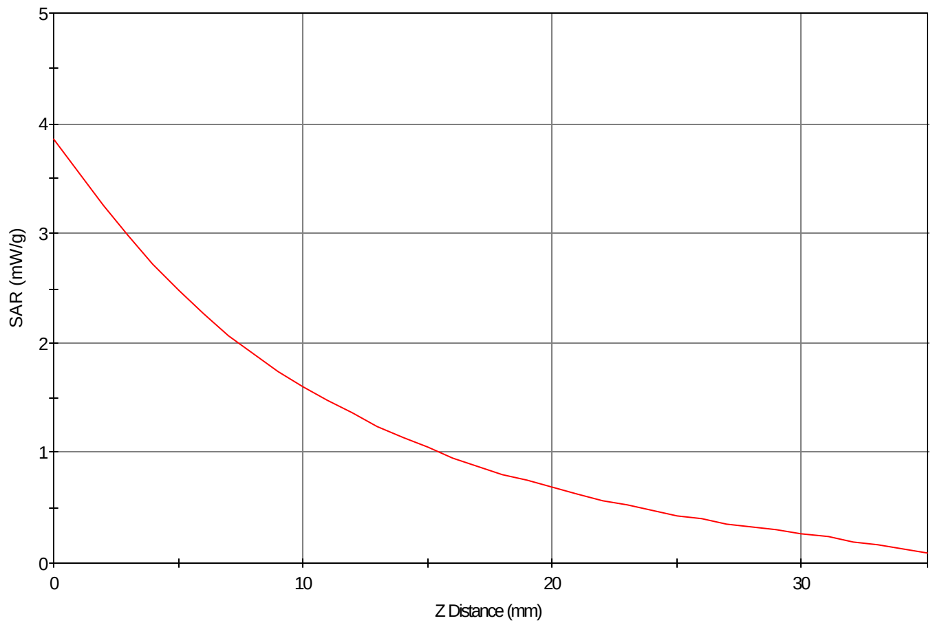
SAR - Z Axis at Hotspot x:-16.0 y:-1.0
