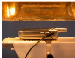
Figure A.10 Body SAR Test Setup -- w/o Belt Clip --
