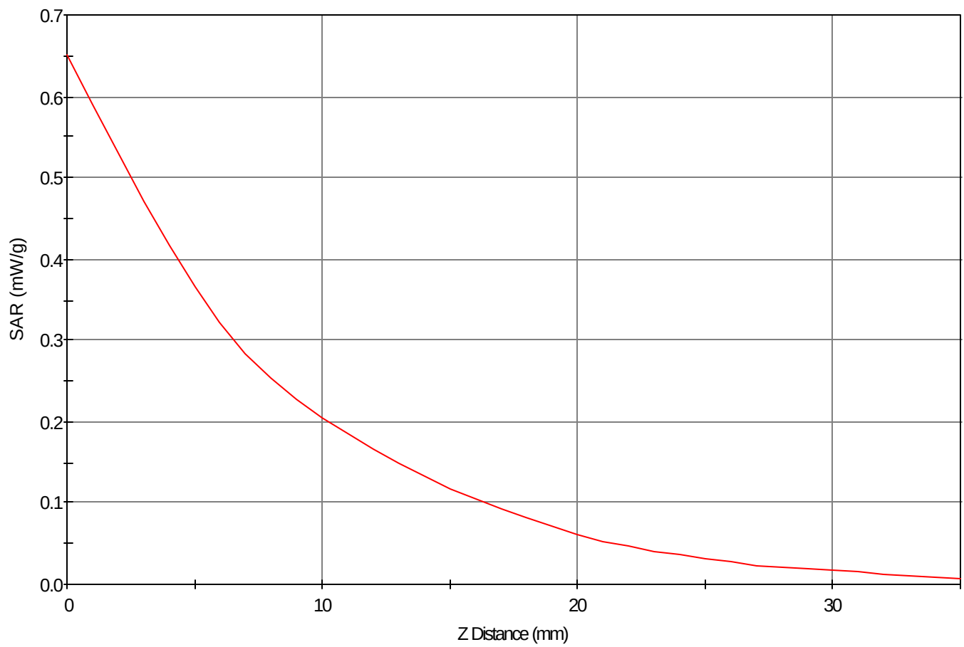
SAR - Z Axis at Hotspot x:65.0 y:2.0
