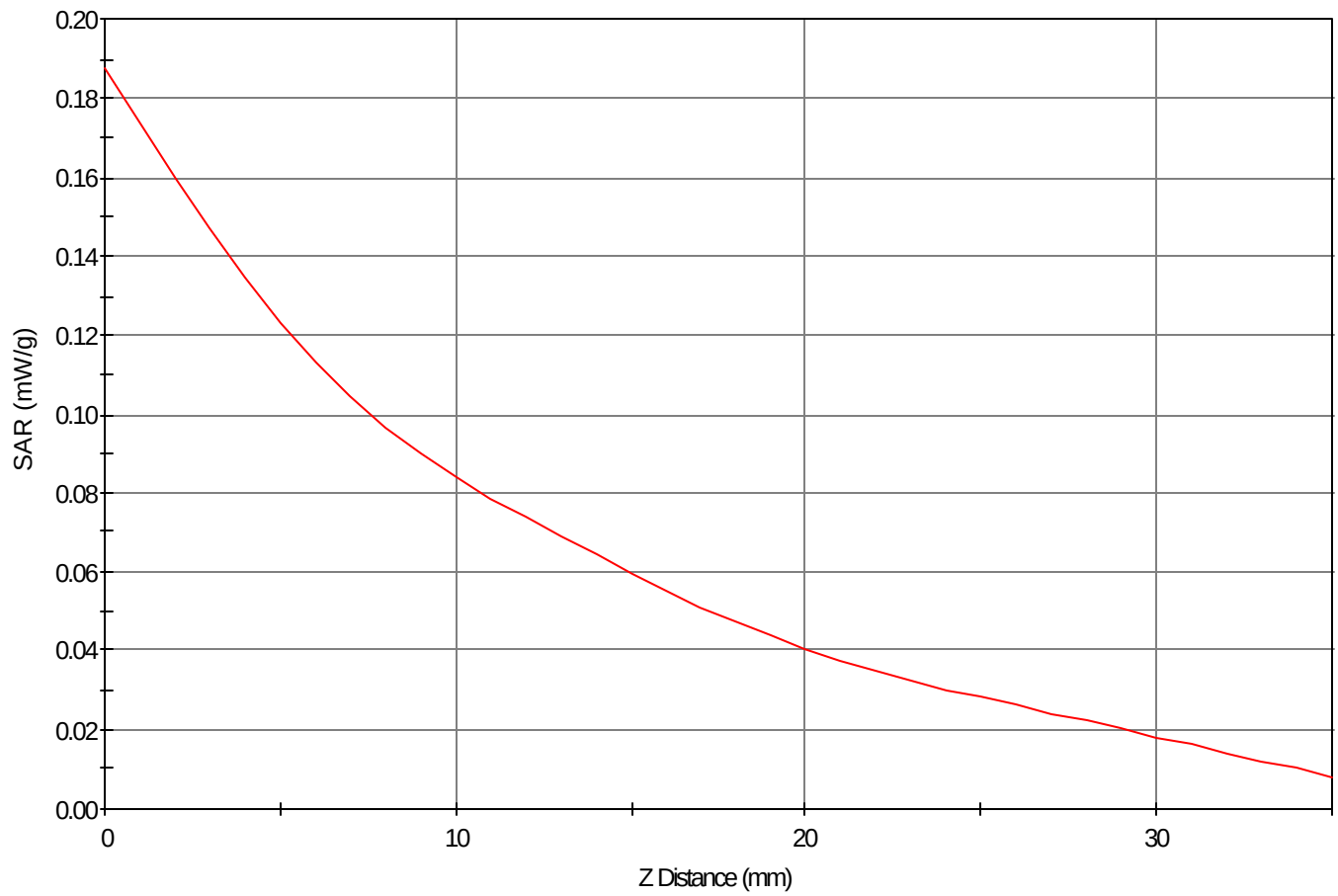
SAR - Z Axis at Hotspot x:87.0 y:7.0
