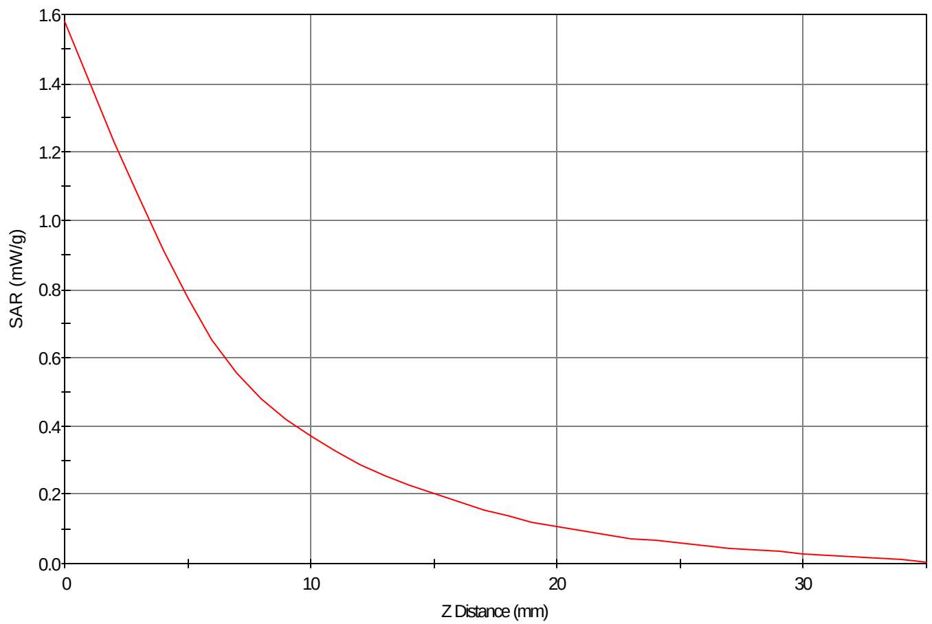
SAR - Z Axis at Hotspot x:-11.0 y:32.0
